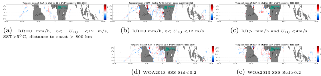
Figure 12: Temporal mean gridded over spatial boxes of size 1^\circ \times 1^\circ of \Delta SSS (SMOS and SMAP SSS L4 OI v1 - 7 Days (LOPS) - TSG (GOSUD-Research-vessel)) for 5 different subdatasets corresponding to:RR=0 mm/h, 3 < U_{10} < 12 m/s, SST>5°C, distance to coast > 800 km (a), RR=0 mm/h, 3 < U_{10} < 12 m/s (b), RR>1mm/h and U_{10} < 4 m/s (c), WOA2013 SSS Std<0.2 (d), WOA2013 SSS Std>0.2 (e).
