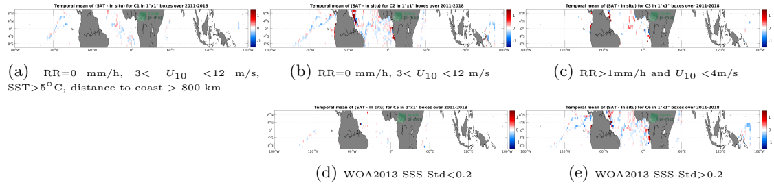
Figure 12: Temporal mean gridded over spatial boxes of size 1^{\circ}\times 1^{\circ} of \Delta SSS (SMOS and SMAP SSS L4 OI v1 - 7 Days (LOPS) - TSG (GOSUD-Research-vessel)) for 5 different subdatasets corresponding to: RR=0 mm/h, 3 < U_{10} < 12 m/s, SST > 5^{\circ}\text{C} , distance to coast > 800 km (a), RR=0 mm/h, 3 < U_{10} < 12 m/s (b), RR > 1 mm/h and U_{10} < 4 m/s (c), WOA2013 SSS Std < 0.2 (d), WOA2013 SSS Std > 0.2 (e).
