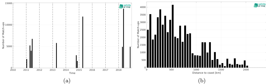
Figure 1: Number of match-ups between TSG (CSIC-UTM) and SMOS and SMAP SSS L4 OI v1 - 7 Days (LOPS) SSS as a function of time (a) and as function of the distance to coast (b) over the Equatorial Ocean 10N-10S Pi-MEP region and for the full satellite product period.
