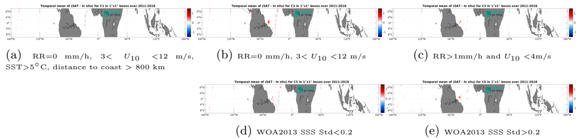
Figure 12: Temporal mean gridded over spatial boxes of size 1^\circ \times 1^\circ of \Delta SSS (SMOS and SMAP SSS L4 OI v1 - 7 Days (LOPS) - TSG (CSIC-UTM)) for 5 different subdatasets corresponding to:RR=0 mm/h, 3 < U_{10} < 12 m/s, SST >5^\circ\text{C} , distance to coast > 800 km (a), RR=0 mm/h, 3 < U_{10} < 12 m/s (b), RR >1 mm/h and U_{10} < 4 m/s (c), WOA2013 SSS Std <0.2 (d), WOA2013 SSS Std >0.2 (e).
