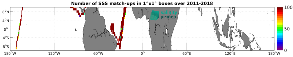
Figure 4: Number of SSS match-ups between TSG (CSIC-UTM) SSS and the SMOS and SMAP SSS L4 OI v1 - 7 Days (LOPS) SSS product for the Equatorial Ocean 10N-10S Pi-MEP region over 1^\circ \times 1^\circ boxes and for the full satellite product period.
