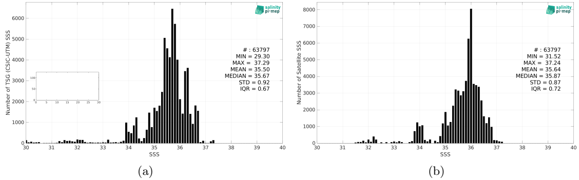
Figure 2: Histograms of SSS from TSG (CSIC-UTM) (a) and SMOS and SMAP SSS L4 OI v1 - 7 Days (LOPS) (b) considering all match-up pairs per bins of 0.1 over the Equatorial Ocean 10N-10S Pi-MEP region and for the full satellite product period.
