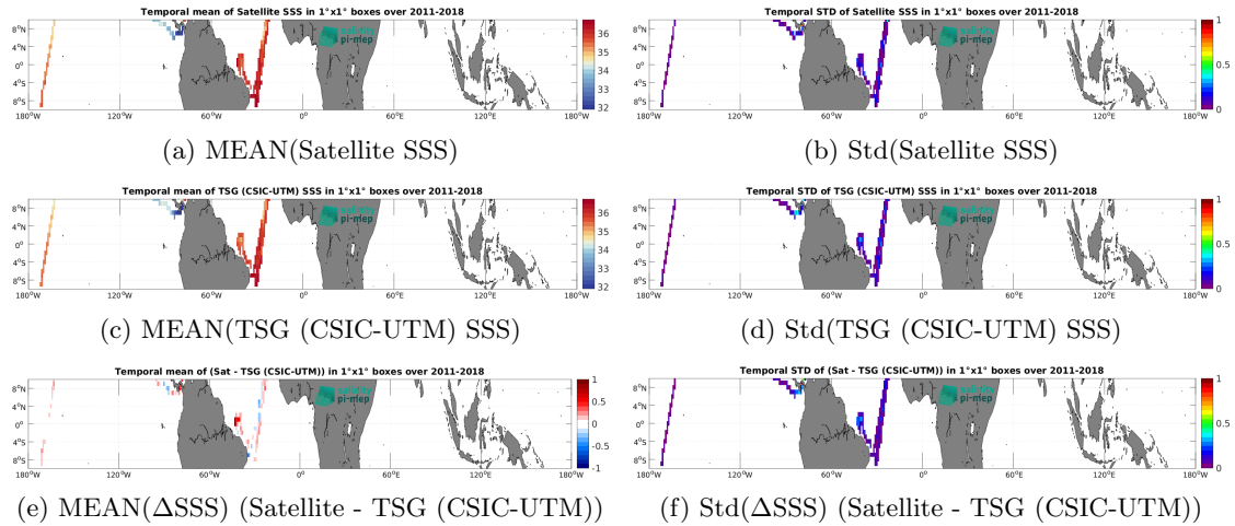
Figure 6: Temporal mean (left) and Std (right) of SSS from SMOS and SMAP SSS L4 OI v1 - 7 Days (LOPS) (top), TSG (CSIC-UTM) (middle), and of \Delta SSS (Satellite - TSG (CSIC-UTM)). Only match-up pairs are used to generate these maps.
