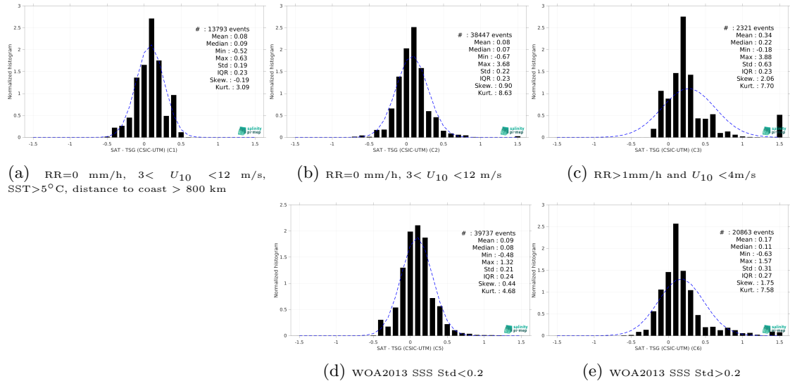
Figure 13: Normalized histogram of \Delta SSS (SMOS and SMAP SSS L4 OI v1 - 7 Days (LOPS) - TSG (CSIC-UTM)) for 5 different subdatasets corresponding to: RR=0 mm/h, 3 < U_{10} < 12 m/s, SST >5^\circ\text{C} , distance to coast > 800 km (a), RR=0 mm/h, 3 < U_{10} < 12 m/s (b), RR >1 mm/h and U_{10} < 4 m/s (c), WOA2013 SSS Std <0.2 (d), WOA2013 SSS Std >0.2 (e).
