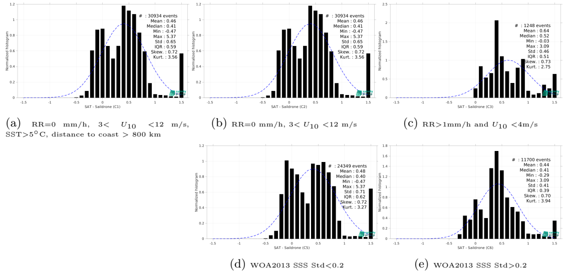
Figure 13: Normalized histogram of \Delta SSS (SMOS and SMAP SSS L4 OI v1 - 7 Days (LOPS) - Saildrone) for 5 different subdatasets corresponding to: RR=0 mm/h, 3 < U_{10} < 12 m/s, SST >5^\circ\text{C} , distance to coast > 800 km (a), RR=0 mm/h, 3 < U_{10} < 12 m/s (b), RR >1 mm/h and U_{10} < 4 m/s (c), WOA2013 SSS Std <0.2 (d), WOA2013 SSS Std >0.2 (e).
