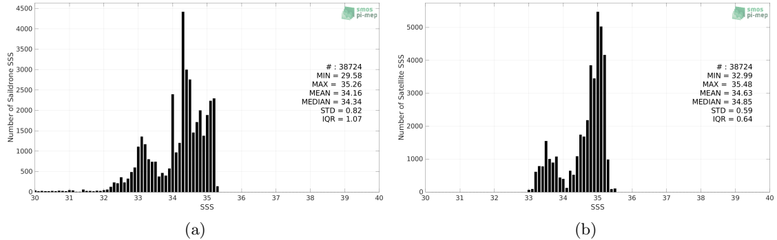
Figure 2: Histograms of SSS from Saildrone (a) and SMOS and SMAP SSS L4 OI v1 - 7 Days (LOPS) (b) considering all match-up pairs per bins of 0.1 over the Equatorial Ocean 10N-10S Pi-MEP region and for the full satellite product period.
