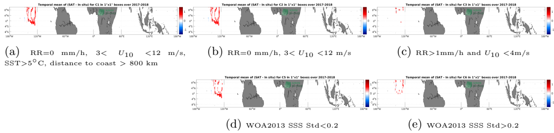
Figure 12: Temporal mean gridded over spatial boxes of size 1^\circ \times 1^\circ of \Delta SSS (SMOS and SMAP SSS L4 OI v1 - 7 Days (LOPS) - Saildrone) for 5 different subdatasets corresponding to: RR=0 mm/h, 3 < U_{10} < 12 m/s, SST>5°C, distance to coast > 800 km (a), RR=0 mm/h, 3 < U_{10} < 12 m/s (b), RR>1mm/h and U_{10} < 4 m/s (c), WOA2013 SSS Std<0.2 (d), WOA2013 SSS Std>0.2 (e).
