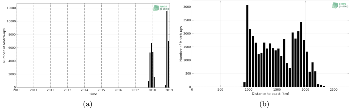
Figure 1: Number of match-ups between Saildrone and SMOS and SMAP SSS L4 OI v1 - 7 Days (LOPS) SSS as a function of time (a) and as function of the distance to coast (b) over the Equatorial Ocean 10N-10S Pi-MEP region and for the full satellite product period.
