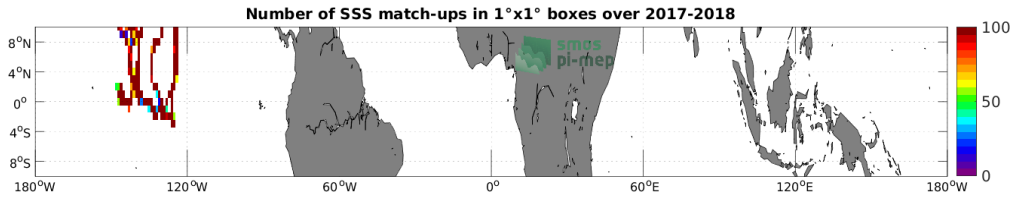
Figure 4: Number of SSS match-ups between Saildrone SSS and the SMOS and SMAP SSS L4 OI v1 - 7 Days (LOPS) SSS product for the Equatorial Ocean 10N-10S Pi-MEP region over 1^\circ \times 1^\circ boxes and for the full satellite product period.
