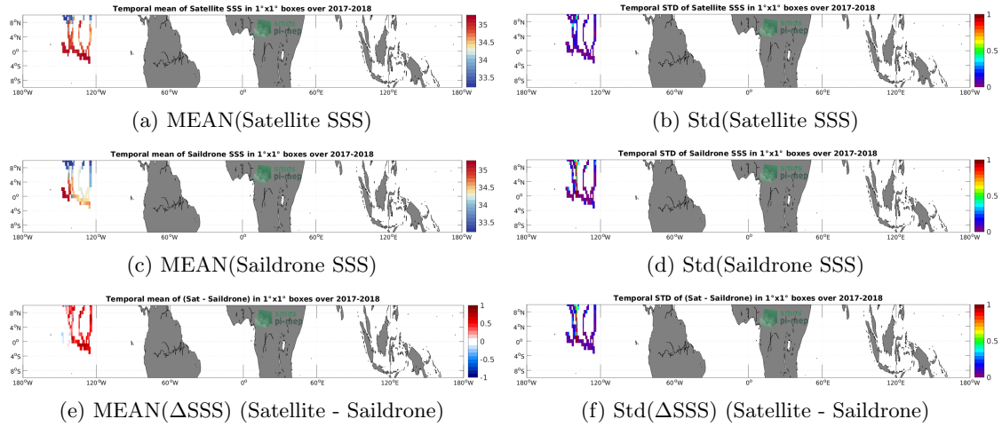
Figure 6: Temporal mean (left) and Std (right) of SSS from SMOS and SMAP SSS L4 OI v1 - 7 Days (LOPS) (top), Saildrone (middle), and of \Delta SSS (Satellite - Saildrone). Only match-up pairs are used to generate these maps.
