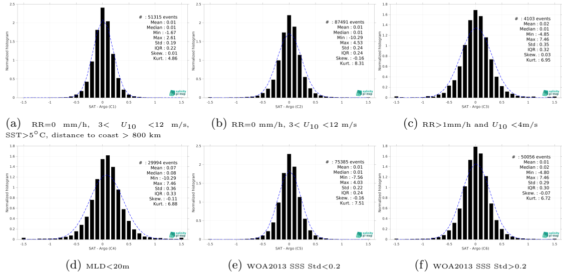
Figure 13: Normalized histogram of \Delta SSS (SMOS and SMAP SSS L4 OI v1 - 7 Days (LOPS) - Argo) for 6 different subdatasets corresponding to: RR=0 mm/h, 3 < U_{10} < 12 m/s, SST > 5°C, distance to coast > 800 km (a), RR=0 mm/h, 3 < U_{10} < 12 m/s (b), RR > 1mm/h and U_{10} < 4 m/s (c), MLD < 20m (d), WOA2013 SSS Std < 0.2 (e), WOA2013 SSS Std > 0.2 (f).
