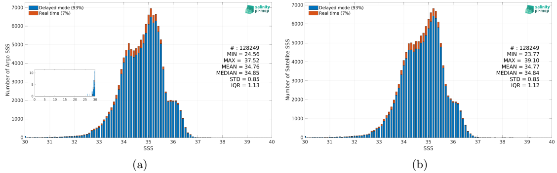
Figure 2: Histograms of SSS from Argo (a) and SMOS and SMAP SSS L4 OI v1 - 7 Days (LOPS) (b) considering all match-up pairs per bins of 0.1 over the Equatorial Ocean 10N-10S Pi-MEP region and for the full satellite product period.
