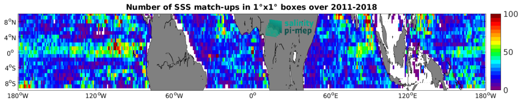
Figure 4: Number of SSS match-ups between Argo SSS and the SMOS and SMAP SSS L4 OI v1 - 7 Days (LOPS) SSS product for the Equatorial Ocean 10N-10S Pi-MEP region over 1^\circ \times 1^\circ boxes and for the full satellite product period.
