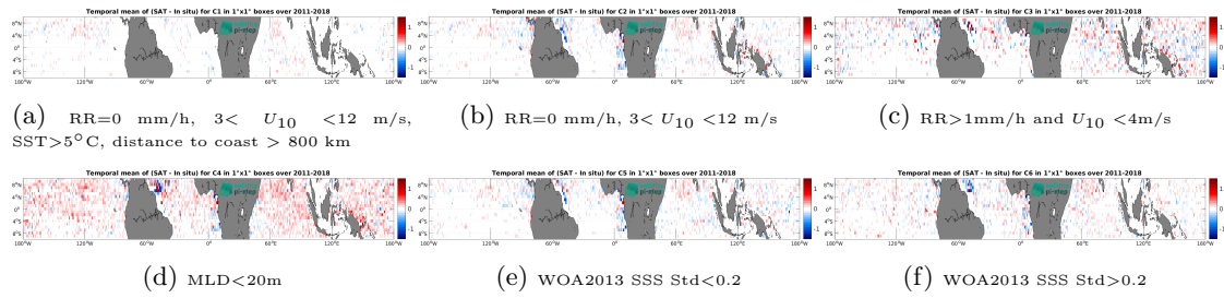
Figure 12: Temporal mean gridded over spatial boxes of size 1^\circ \times 1^\circ of \Delta SSS (SMOS and SMAP SSS L4 OI v1 - 7 Days (LOPS) - Argo) for 6 different subdatasets corresponding to:RR=0 mm/h, 3 < U_{10} < 12 m/s, SST >5^\circ C, distance to coast > 800 km (a), RR=0 mm/h, 3 < U_{10} < 12 m/s (b), RR >1 mm/h and U_{10} < 4 m/s (c),MLD <20 m (d),WOA2013 SSS Std <0.2 (e),WOA2013 SSS Std >0.2 (f).
