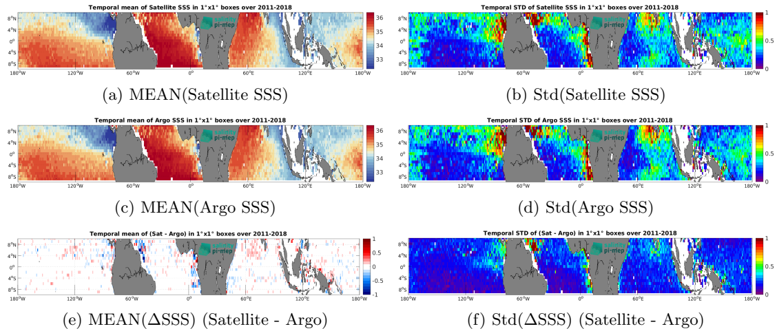
Figure 6: Temporal mean (left) and Std (right) of SSS from SMOS and SMAP SSS L4 OI v1 - 7 Days (LOPS) (top), Argo (middle), and of \Delta SSS (Satellite - Argo). Only match-up pairs are used to generate these maps.
