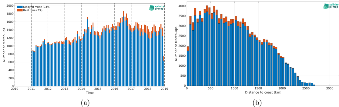
Figure 1: Number of match-ups between Argo and SMOS and SMAP SSS L4 OI v1 - 7 Days (LOPS) SSS as a function of time (a) and as function of the distance to coast (b) over the Equatorial Ocean 10N-10S Pi-MEP region and for the full satellite product period.
