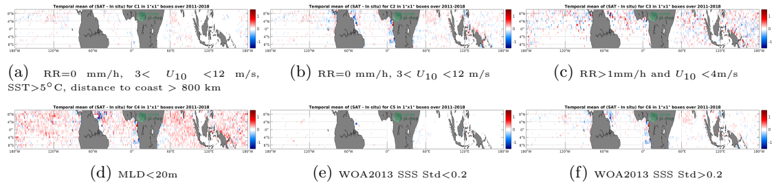
Figure 12: Temporal mean gridded over spatial boxes of size 1^\circ \times 1^\circ of \Delta SSS (SMOS and SMAP SSS L4 OI v1 - 7 Days (LOPS) - Argo) for 6 different subdatasets corresponding to:RR=0 mm/h, 3 < U_{10} < 12 m/s, SST >5^\circ C, distance to coast > 800 km (a), RR=0 mm/h, 3 < U_{10} < 12 m/s (b), RR >1 mm/h and U_{10} < 4 m/s (c),MLD <20 m (d),WOA2013 SSS Std <0.2 (e),WOA2013 SSS Std >0.2 (f).
