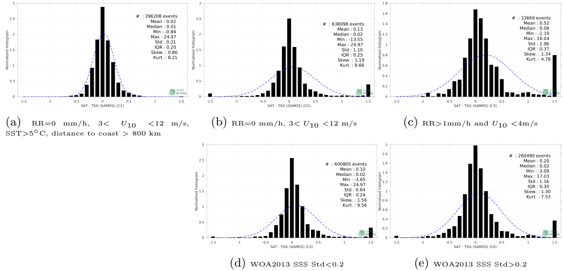
Figure 13: Normalized histogram of \Delta SSS (SMOS SSS L4 v1 - Weekly (CMEMS-CNR) - TSG (SAMOS)) for 5 different subdatasets corresponding to: RR=0 mm/h, 3 < U_{10} < 12 m/s, SST >5^\circ\text{C} , distance to coast > 800 km (a), RR=0 mm/h, 3 < U_{10} < 12 m/s (b), RR >1 mm/h and U_{10} < 4 m/s (c), WOA2013 SSS Std <0.2 (d), WOA2013 SSS Std >0.2 (e).
