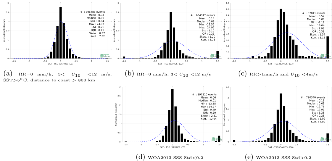
Figure 13: Normalized histogram of \Delta SSS (SMOS SSS L4 v1 - Weekly (CMEMS-CNR) - TSG (SAMOS)) for 5 different subdatasets corresponding to: RR=0 mm/h, 3 < U_{10} < 12 m/s, SST >5^\circ\text{C} , distance to coast > 800 km (a), RR=0 mm/h, 3 < U_{10} < 12 m/s (b), RR >1 mm/h and U_{10} < 4 m/s (c), WOA2013 SSS Std <0.2 (d), WOA2013 SSS Std >0.2 (e).
