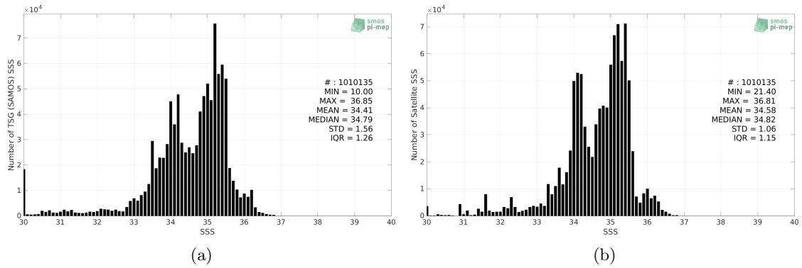
Figure 2: Histograms of SSS from TSG (SAMOS) (a) and SMOS SSS L4 v1 - Weekly (CMEMS-CNR) (b) considering all match-up pairs per bins of 0.1 over the Equatorial Ocean 10N-10S Pi-MEP region and for the full satellite product period.
