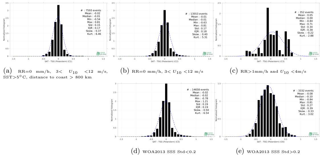
Figure 13: Normalized histogram of \Delta SSS (SMOS SSS L4 v1 - Weekly (CMEMS-CNR) - TSG (Polarstern)) for 5 different subdatasets corresponding to: RR=0 mm/h, 3 < U_{10} < 12 m/s, SST >5^\circ\text{C} , distance to coast > 800 km (a), RR=0 mm/h, 3 < U_{10} < 12 m/s (b), RR >1 mm/h and U_{10} < 4 m/s (c), WOA2013 SSS Std <0.2 (d), WOA2013 SSS Std >0.2 (e).
