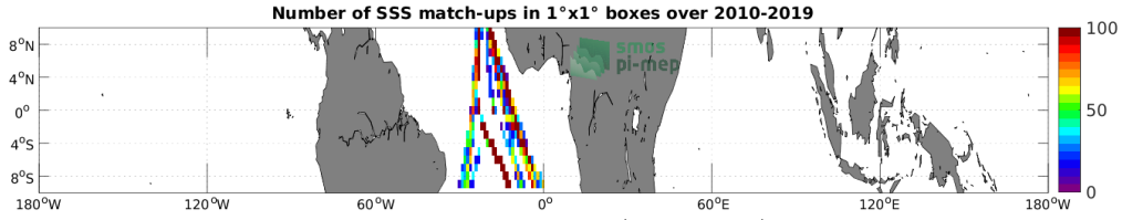
Figure 4: Number of SSS match-ups between TSG (Polarstern) SSS and the SMOS SSS L4 v1 - Weekly (CMEMS-CNR) SSS product for the Equatorial Ocean 10N-10S Pi-MEP region over 1^\circ \times 1^\circ boxes and for the full satellite product period.
