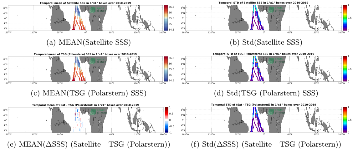
Figure 6: Temporal mean (left) and Std (right) of SSS from SMOS SSS L4 v1 - Weekly (CMEMS-CNR) (top), TSG (Polarstern) (middle), and of \Delta SSS (Satellite - TSG (Polarstern)). Only match-up pairs are used to generate these maps.
