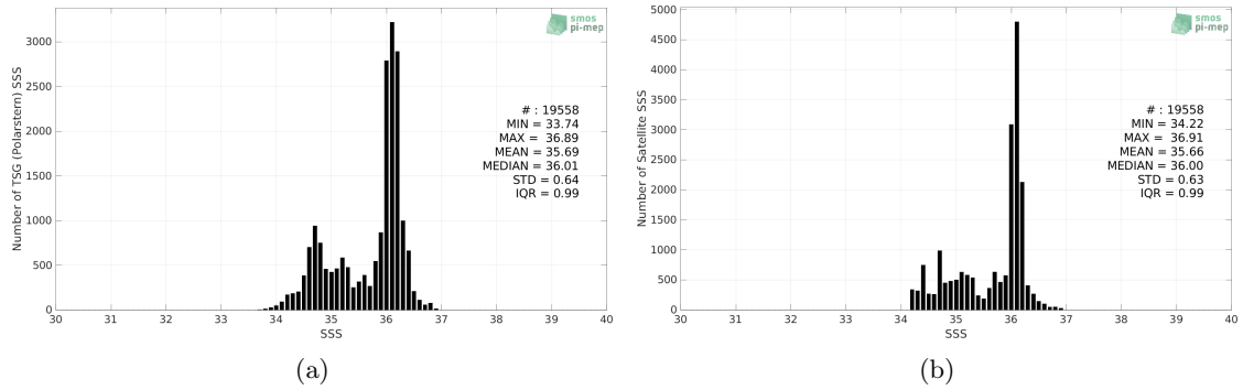
Figure 2: Histograms of SSS from TSG (Polarstern) (a) and SMOS SSS L4 v1 - Weekly (CMEMS-CNR) (b) considering all match-up pairs per bins of 0.1 over the Equatorial Ocean 10N-10S Pi-MEP region and for the full satellite product period.
