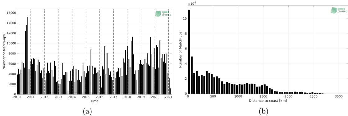
Figure 1: Number of match-ups between TSG (LEGOS-DM) and SMOS SSS L4 v1 - Weekly (CMEMS-CNR) SSS as a function of time (a) and as function of the distance to coast (b) over the Equatorial Ocean 10N-10S Pi-MEP region and for the full satellite product period.
