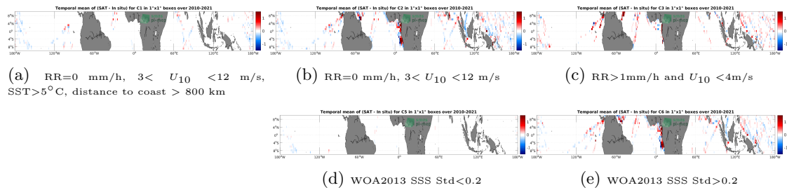
Figure 12: Temporal mean gridded over spatial boxes of size 1^\circ \times 1^\circ of \Delta SSS (SMOS SSS L4 v1 - Weekly (CMEMS-CNR) - TSG (LEGOS-DM)) for 5 different subdatasets corresponding to: RR=0 mm/h, 3 < U_{10} < 12 m/s, SST >5^\circ\text{C} , distance to coast > 800 km (a), RR=0 mm/h, 3 < U_{10} < 12 m/s (b), RR >1 mm/h and U_{10} < 4 m/s (c), WOA2013 SSS Std <0.2 (d), WOA2013 SSS Std >0.2 (e).
