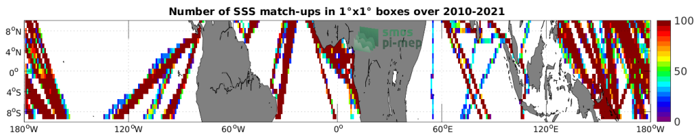
Figure 4: Number of SSS match-ups between TSG (LEGOS-DM) SSS and the SMOS SSS L4 v1 - Weekly (CMEMS-CNR) SSS product for the Equatorial Ocean 10N-10S Pi-MEP region over 1^\circ \times 1^\circ boxes and for the full satellite product period.
