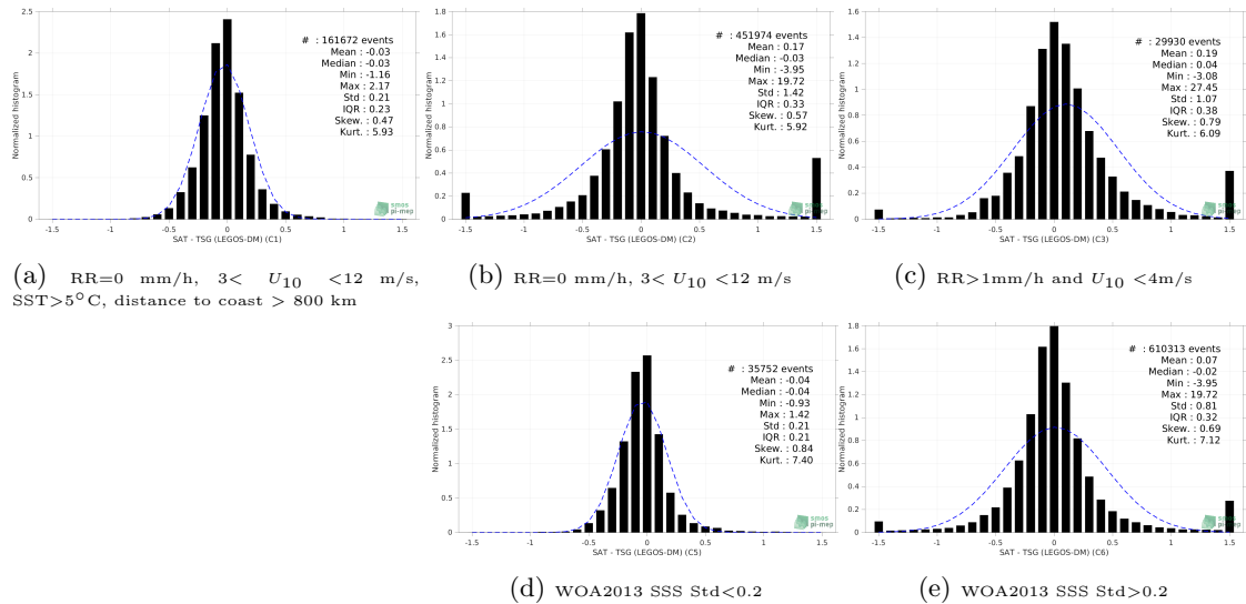
Figure 13: Normalized histogram of \Delta SSS (SMOS SSS L4 v1 - Weekly (CMEMS-CNR) - TSG (LEGOS-DM)) for 5 different subdatasets corresponding to: RR=0 mm/h, 3 < U_{10} < 12 m/s, SST >5^\circ\text{C} , distance to coast > 800 km (a), RR=0 mm/h, 3 < U_{10} < 12 m/s (b), RR >1 mm/h and U_{10} < 4 m/s (c), WOA2013 SSS Std <0.2 (d), WOA2013 SSS Std >0.2 (e).
