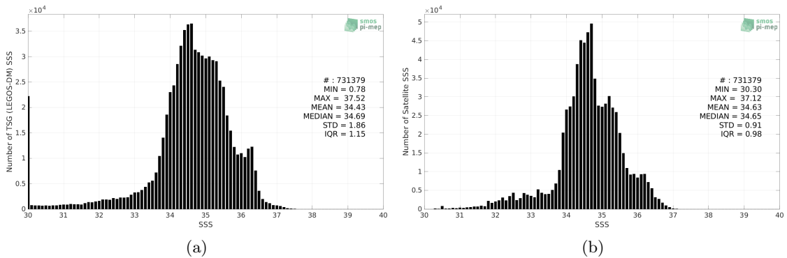
Figure 2: Histograms of SSS from TSG (LEGOS-DM) (a) and SMOS SSS L4 v1 - Weekly (CMEMS-CNR) (b) considering all match-up pairs per bins of 0.1 over the Equatorial Ocean 10N-10S Pi-MEP region and for the full satellite product period.
