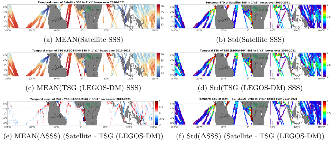
Figure 6: Temporal mean (left) and Std (right) of SSS from SMOS SSS L4 v1 - Weekly (CMEMS-CNR) (top), TSG (LEGOS-DM) (middle), and of \Delta SSS (Satellite - TSG (LEGOS-DM)). Only match-up pairs are used to generate these maps.
