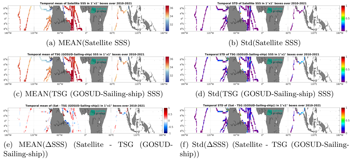
Figure 6: Temporal mean (left) and Std (right) of SSS from SMOS SSS L4 v1 - Weekly (CMEMS-CNR) (top), TSG (GOSUD-Sailing-ship) (middle), and of \Delta SSS (Satellite - TSG (GOSUD-Sailing-ship)). Only match-up pairs are used to generate these maps.
