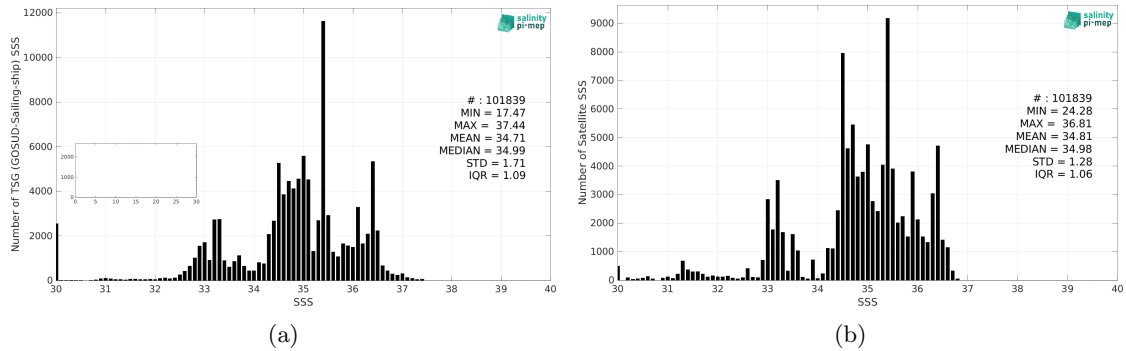
Figure 2: Histograms of SSS from TSG (GOSUD-Sailing-ship) (a) and SMOS SSS L4 v1 - Weekly (CMEMS-CNR) (b) considering all match-up pairs per bins of 0.1 over the Equatorial Ocean 10N-10S Pi-MEP region and for the full satellite product period.
