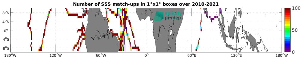
Figure 4: Number of SSS match-ups between TSG (GOSUD-Sailing-ship) SSS and the SMOS SSS L4 v1 - Weekly (CMEMS-CNR) SSS product for the Equatorial Ocean 10N-10S Pi-MEP region over 1^\circ \times 1^\circ boxes and for the full satellite product period.
