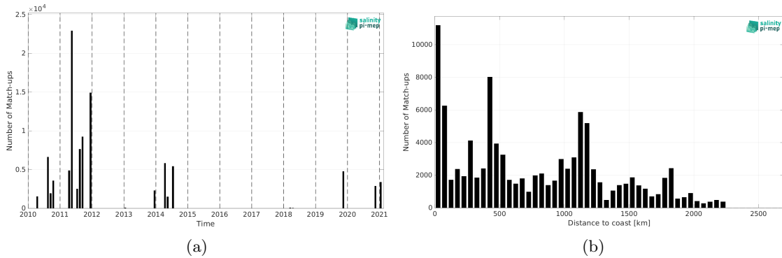
Figure 1: Number of match-ups between TSG (GOSUD-Sailing-ship) and SMOS SSS L4 v1 - Weekly (CMEMS-CNR) SSS as a function of time (a) and as function of the distance to coast (b) over the Equatorial Ocean 10N-10S Pi-MEP region and for the full satellite product period.
