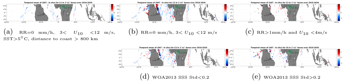
Figure 12: Temporal mean gridded over spatial boxes of size 1^{\circ}\times 1^{\circ} of \Delta SSS (SMOS SSS L4 v1 - Weekly (CMEMS-CNR) - TSG (GOSUD-Research-vessel)) for 5 different subdatasets corresponding to:RR=0 mm/h, 3 < U_{10} < 12 m/s, SST >5^{\circ}\text{C} , distance to coast > 800 km (a), RR=0 mm/h, 3 < U_{10} < 12 m/s (b), RR >1 mm/h and U_{10} < 4 m/s (c), WOA2013 SSS Std <0.2 (d), WOA2013 SSS Std >0.2 (e).
