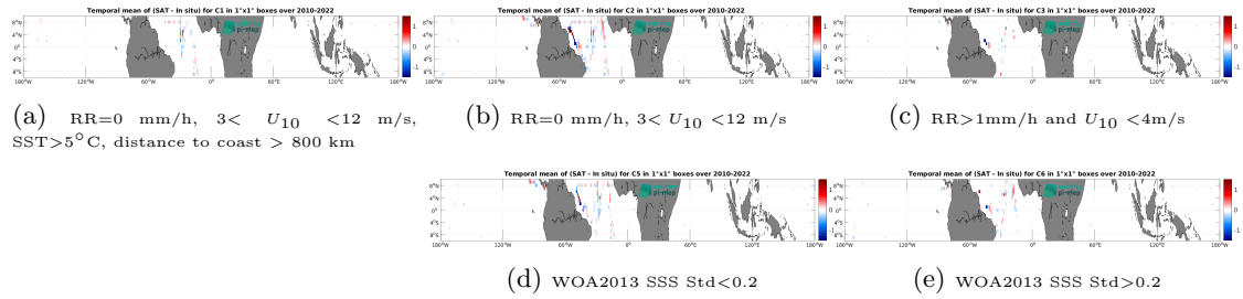
Figure 12: Temporal mean gridded over spatial boxes of size 1^\circ \times 1^\circ of \Delta SSS (SMOS SSS L4 v1 - Weekly (CMEMS-CNR) - TSG (CSIC-UTM)) for 5 different subdatasets corresponding to: RR=0 mm/h, 3 < U_{10} < 12 m/s, SST >5^\circ\text{C} , distance to coast > 800 km (a), RR=0 mm/h, 3 < U_{10} < 12 m/s (b), RR >1 mm/h and U_{10} < 4 m/s (c), WOA2013 SSS Std <0.2 (d), WOA2013 SSS Std >0.2 (e).
