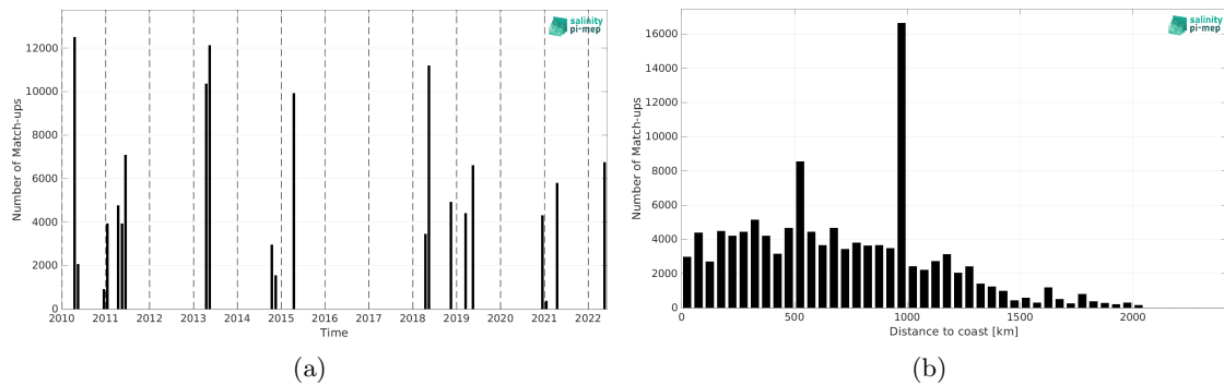
Figure 1: Number of match-ups between TSG (CSIC-UTM) and SMOS SSS L4 v1 - Weekly (CMEMS-CNR) SSS as a function of time (a) and as function of the distance to coast (b) over the Equatorial Ocean 10N-10S Pi-MEP region and for the full satellite product period.
