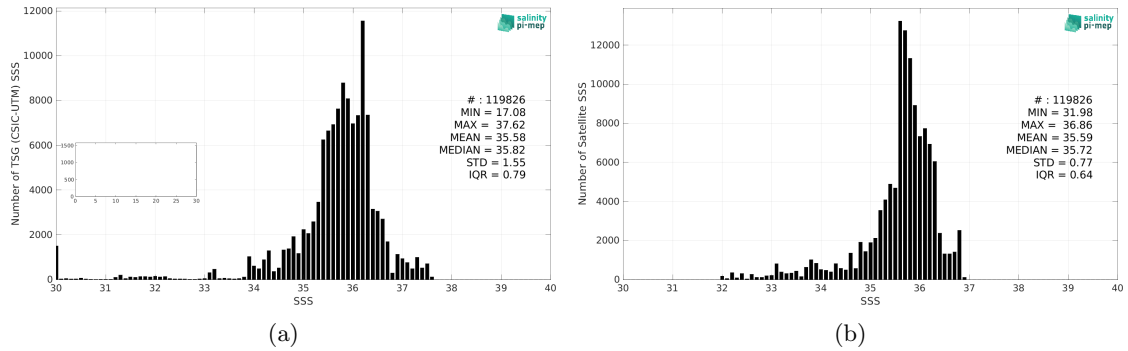
Figure 2: Histograms of SSS from TSG (CSIC-UTM) (a) and SMOS SSS L4 v1 - Weekly (CMEMS-CNR) (b) considering all match-up pairs per bins of 0.1 over the Equatorial Ocean 10N-10S Pi-MEP region and for the full satellite product period.
