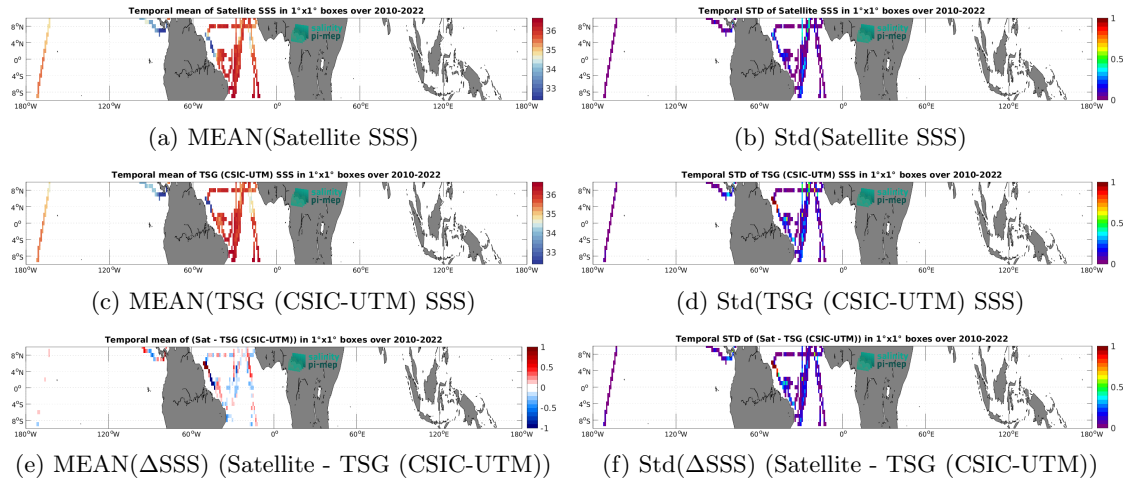
Figure 6: Temporal mean (left) and Std (right) of SSS from SMOS SSS L4 v1 - Weekly (CMEMS-CNR) (top), TSG (CSIC-UTM) (middle), and of \Delta SSS (Satellite - TSG (CSIC-UTM)). Only match-up pairs are used to generate these maps.
