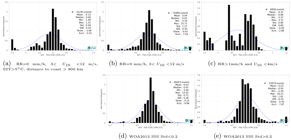
Figure 13: Normalized histogram of \Delta SSS (SMOS SSS L4 v1 - Weekly (CMEMS-CNR) - TSG (CSIC-UTM)) for 5 different subdatasets corresponding to: RR=0 mm/h, 3 < U_{10} < 12 m/s, SST >5^\circ\text{C} , distance to coast > 800 km (a), RR=0 mm/h, 3 < U_{10} < 12 m/s (b), RR >1 mm/h and U_{10} < 4 m/s (c), WOA2013 SSS Std <0.2 (d), WOA2013 SSS Std >0.2 (e).
