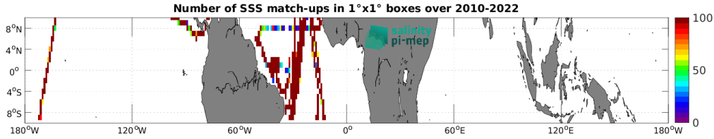
Figure 4: Number of SSS match-ups between TSG (CSIC-UTM) SSS and the SMOS SSS L4 v1 - Weekly (CMEMS-CNR) SSS product for the Equatorial Ocean 10N-10S Pi-MEP region over 1^\circ \times 1^\circ boxes and for the full satellite product period.
