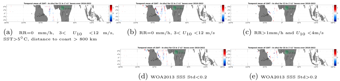
Figure 12: Temporal mean gridded over spatial boxes of size 1^\circ \times 1^\circ of \Delta SSS (SMOS SSS L4 v1 - Weekly (CMEMS-CNR) - TSG (CSIC-UTM)) for 5 different subdatasets corresponding to: RR=0 mm/h, 3 < U_{10} < 12 m/s, SST>5°C, distance to coast > 800 km (a), RR=0 mm/h, 3 < U_{10} < 12 m/s (b), RR>1mm/h and U_{10} < 4 m/s (c), WOA2013 SSS Std<0.2 (d), WOA2013 SSS Std>0.2 (e).
