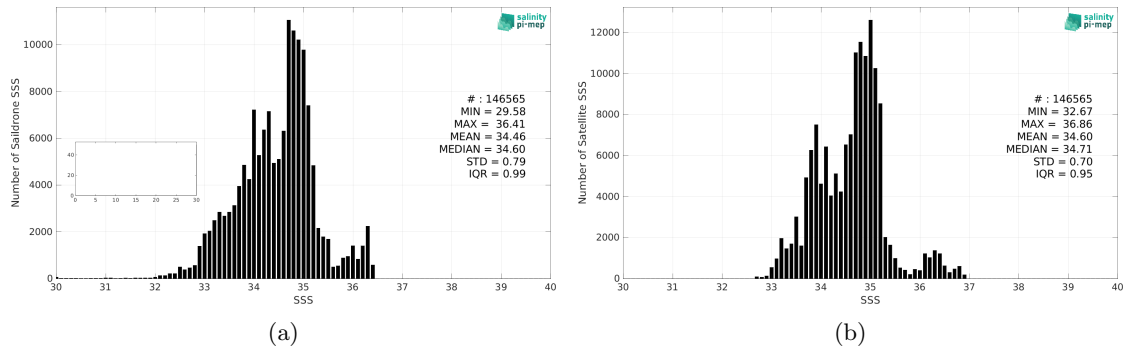
Figure 2: Histograms of SSS from Saildrone (a) and SMOS SSS L4 v1 - Weekly (CMEMS-CNR) (b) considering all match-up pairs per bins of 0.1 over the Equatorial Ocean 10N-10S Pi-MEP region and for the full satellite product period.
