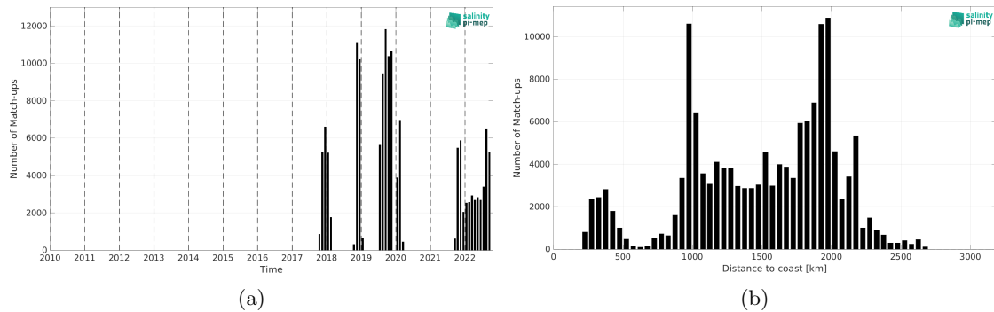
Figure 1: Number of match-ups between Saildrone and SMOS SSS L4 v1 - Weekly (CMEMS-CNR) SSS as a function of time (a) and as function of the distance to coast (b) over the Equatorial Ocean 10N-10S Pi-MEP region and for the full satellite product period.
