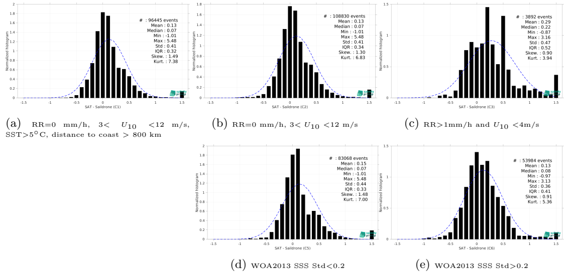
Figure 13: Normalized histogram of \Delta SSS (SMOS SSS L4 v1 - Weekly (CMEMS-CNR) - Saildrone) for 5 different subdatasets corresponding to: RR=0 mm/h, 3 < U_{10} < 12 m/s, SST > 5^\circ C , distance to coast > 800 km (a), RR=0 mm/h, 3 < U_{10} < 12 m/s (b), RR > 1 mm/h and U_{10} < 4 m/s (c), WOA2013 SSS Std < 0.2 (d), WOA2013 SSS Std > 0.2 (e).
