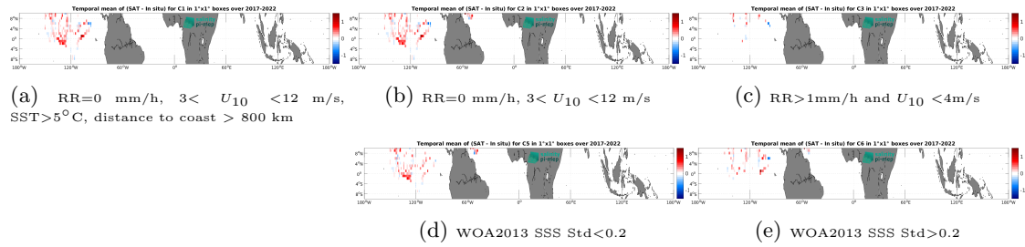
Figure 12: Temporal mean gridded over spatial boxes of size 1^\circ \times 1^\circ of \Delta SSS (SMOS SSS L4 v1 - Weekly (CMEMS-CNR) - Saildrone) for 5 different subdatasets corresponding to: RR=0 mm/h, 3 < U_{10} < 12 m/s, SST > 5^\circ C , distance to coast > 800 km (a), RR=0 mm/h, 3 < U_{10} < 12 m/s (b), RR > 1 mm/h and U_{10} < 4 m/s (c), WOA2013 SSS Std < 0.2 (d), WOA2013 SSS Std > 0.2 (e).
