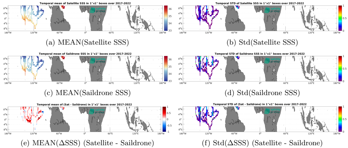
Figure 6: Temporal mean (left) and Std (right) of SSS from SMOS SSS L4 v1 - Weekly (CMEMS-CNR) (top), Saildrone (middle), and of \Delta SSS (Satellite - Saildrone). Only match-up pairs are used to generate these maps.
