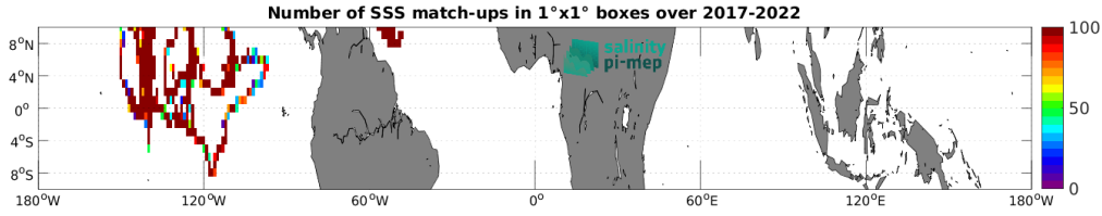
Figure 4: Number of SSS match-ups between Saildrone SSS and the SMOS SSS L4 v1 - Weekly (CMEMS-CNR) SSS product for the Equatorial Ocean 10N-10S Pi-MEP region over 1^\circ \times 1^\circ boxes and for the full satellite product period.
