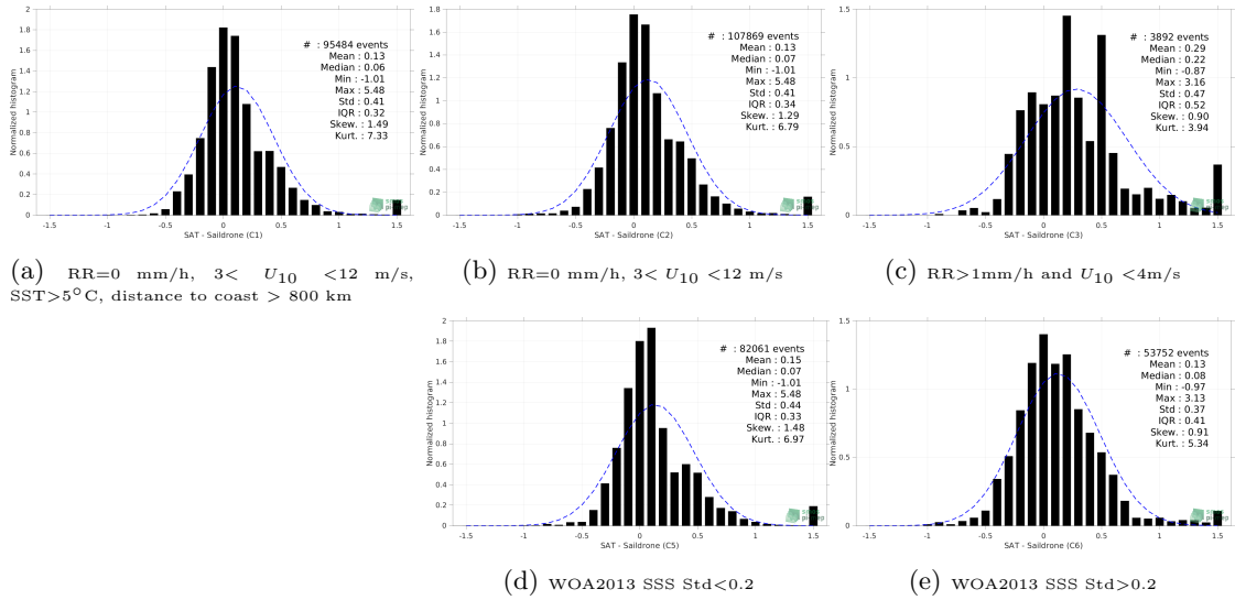
Figure 13: Normalized histogram of \Delta SSS (SMOS SSS L4 v1 - Weekly (CMEMS-CNR) - Saildrone) for 5 different subdatasets corresponding to: RR=0 mm/h, 3 < U_{10} < 12 m/s, SST >5^\circ\text{C} , distance to coast > 800 km (a), RR=0 mm/h, 3 < U_{10} < 12 m/s (b), RR >1 mm/h and U_{10} < 4 m/s (c), WOA2013 SSS Std <0.2 (d), WOA2013 SSS Std >0.2 (e).
