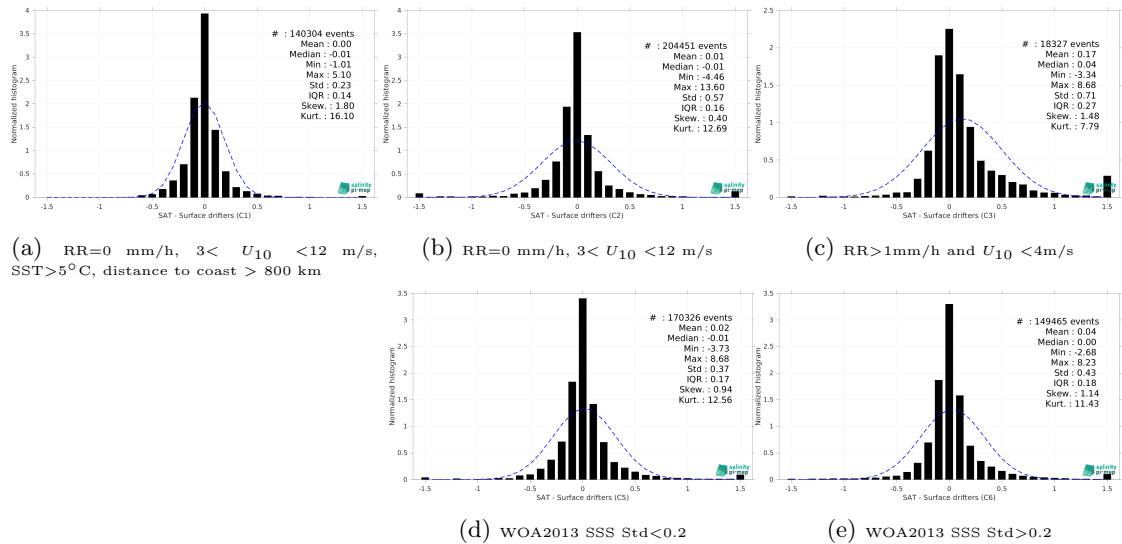
Figure 12: Normalized histogram of \Delta SSS (SMOS SSS L4 v1 - Weekly (CMEMS-CNR) - Surface drifters) for 5 different subdatasets corresponding to: RR=0 mm/h, 3 < U_{10} < 12 m/s, SST >5^\circ C, distance to coast > 800 km (a), RR=0 mm/h, 3 < U_{10} < 12 m/s (b), RR >1 mm/h and U_{10} < 4 m/s (c), WOA2013 SSS Std <0.2 (d), WOA2013 SSS Std >0.2 (e).
