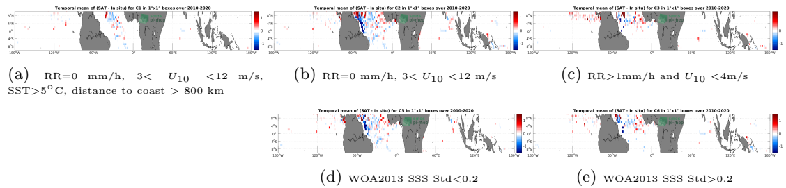
Figure 11: Temporal mean gridded over spatial boxes of size 1^\circ \times 1^\circ of \Delta SSS (SMOS SSS L4 v1 - Weekly (CMEMS-CNR) - Surface drifters) for 5 different subdatasets corresponding to: RR=0 mm/h, 3 < U_{10} < 12 m/s, SST > 5^\circ C , distance to coast > 800 km (a), RR=0 mm/h, 3 < U_{10} < 12 m/s (b), RR>1mm/h and U_{10} < 4 m/s (c), WOA2013 SSS Std<0.2 (d), WOA2013 SSS Std>0.2 (e).
