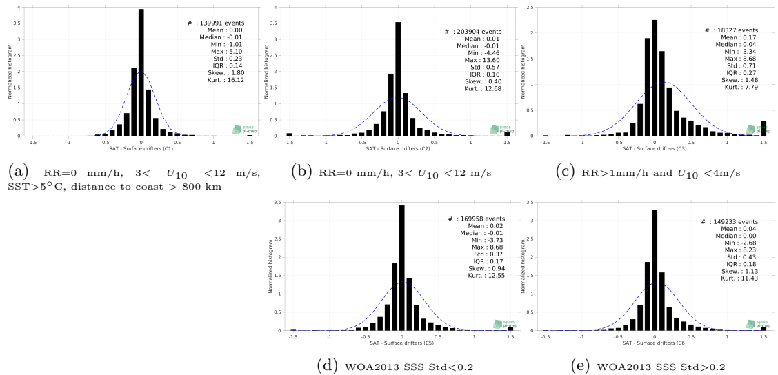
Figure 12: Normalized histogram of \Delta SSS (SMOS SSS L4 v1 - Weekly (CMEMS-CNR) - Surface drifters) for 5 different subdatasets corresponding to: RR=0 mm/h, 3 < U_{10} < 12 m/s, SST > 5^\circ C , distance to coast > 800 km (a), RR=0 mm/h, 3 < U_{10} < 12 m/s (b), RR>1mm/h and U_{10} < 4 m/s (c), WOA2013 SSS Std<0.2 (d), WOA2013 SSS Std>0.2 (e).
