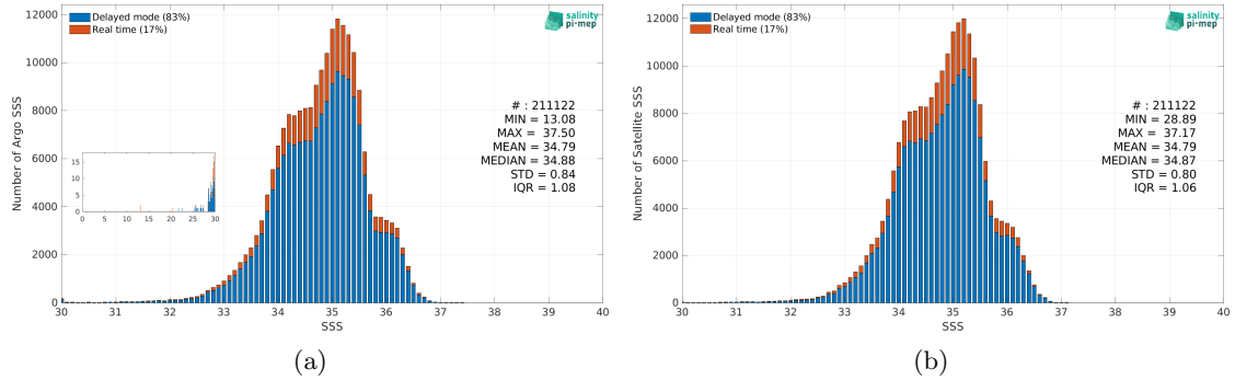
Figure 2: Histograms of SSS from Argo (a) and SMOS SSS L4 v1 - Weekly (CMEMS-CNR) (b) considering all match-up pairs per bins of 0.1 over the Equatorial Ocean 10N-10S Pi-MEP region and for the full satellite product period.
