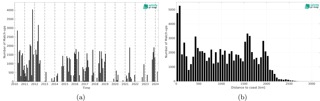
Figure 2: Number of match-ups between TSG (SAMOS) and SMOS SSS L4 v1 - Monthly (CMEMS-CNR) SSS as a function of time (a) and as function of the distance to coast (b) over the Equatorial Ocean 10N-10S Pi-MEP region and for the full satellite product period.
