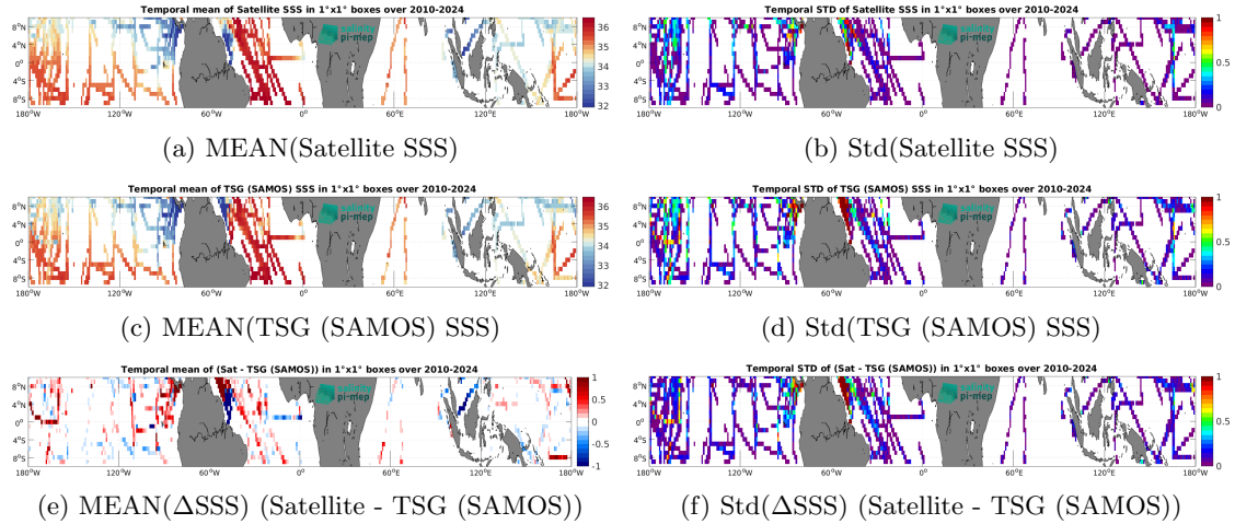
Figure 7: Temporal mean (left) and Std (right) of SSS from SMOS SSS L4 v1 - Monthly (CMEMS-CNR) (top), TSG (SAMOS) (middle), and of \Delta SSS (Satellite - TSG (SAMOS)). Only match-up pairs are used to generate these maps.
