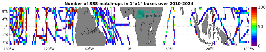
Figure 5: Number of SSS match-ups between TSG (SAMOS) SSS and the SMOS SSS L4 v1 - Monthly (CMEMS-CNR) SSS product for the Equatorial Ocean 10N-10S Pi-MEP region over 1^\circ \times 1^\circ boxes and for the full satellite product period.
