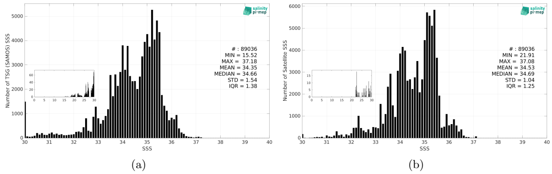
Figure 3: Histograms of SSS from TSG (SAMOS) (a) and SMOS SSS L4 v1 - Monthly (CMEMS-CNR) (b) considering all match-up pairs per bins of 0.1 over the Equatorial Ocean 10N-10S Pi-MEP region and for the full satellite product period.
