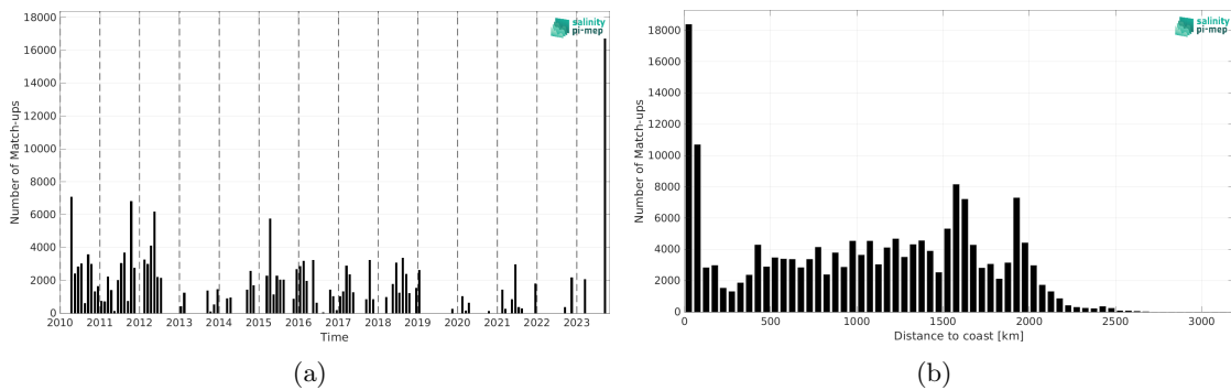
Figure 1: Number of match-ups between TSG (SAMOS) and SMOS SSS L4 v1 - Monthly (CMEMS-CNR) SSS as a function of time (a) and as function of the distance to coast (b) over the Equatorial Ocean 10N-10S Pi-MEP region and for the full satellite product period.
