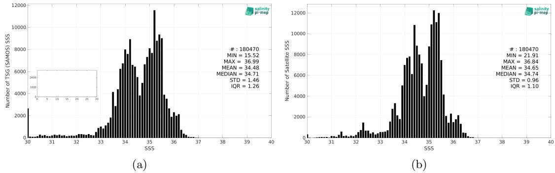
Figure 2: Histograms of SSS from TSG (SAMOS) (a) and SMOS SSS L4 v1 - Monthly (CMEMS-CNR) (b) considering all match-up pairs per bins of 0.1 over the Equatorial Ocean 10N-10S Pi-MEP region and for the full satellite product period.
