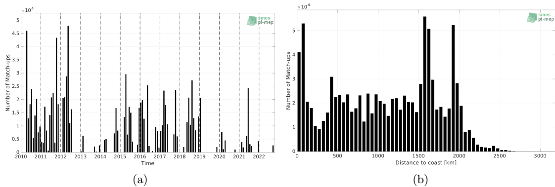
Figure 1: Number of match-ups between TSG (SAMOS) and SMOS SSS L4 v1 - Monthly (CMEMS-CNR) SSS as a function of time (a) and as function of the distance to coast (b) over the Equatorial Ocean 10N-10S Pi-MEP region and for the full satellite product period.
