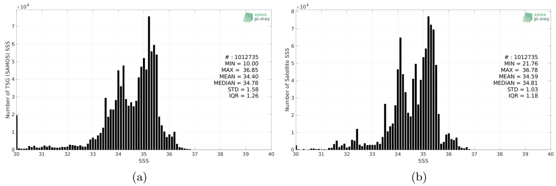
Figure 2: Histograms of SSS from TSG (SAMOS) (a) and SMOS SSS L4 v1 - Monthly (CMEMS-CNR) (b) considering all match-up pairs per bins of 0.1 over the Equatorial Ocean 10N-10S Pi-MEP region and for the full satellite product period.
