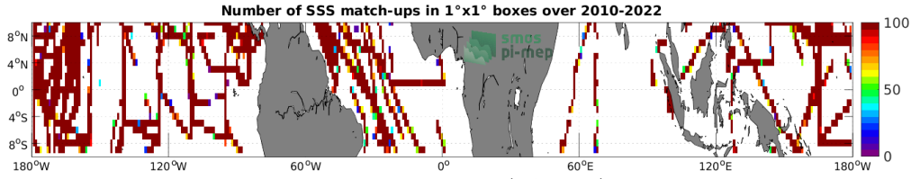
Figure 4: Number of SSS match-ups between TSG (SAMOS) SSS and the SMOS SSS L4 v1 - Monthly (CMEMS-CNR) SSS product for the Equatorial Ocean 10N-10S Pi-MEP region over 1^\circ \times 1^\circ boxes and for the full satellite product period.
