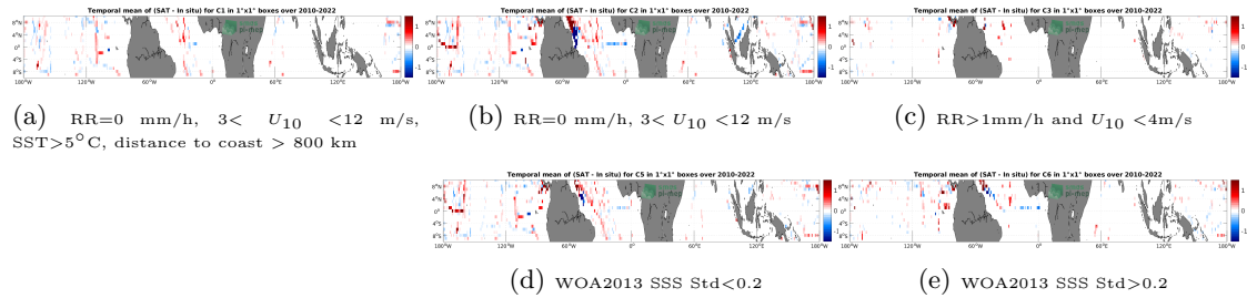
Figure 12: Temporal mean gridded over spatial boxes of size 1^\circ \times 1^\circ of \Delta SSS (SMOS SSS L4 v1 - Monthly (CMEMS-CNR) - TSG (SAMOS)) for 5 different subdatasets corresponding to:RR=0 mm/h, 3 < U_{10} < 12 m/s, SST >5^\circ C, distance to coast > 800 km (a), RR=0 mm/h, 3 < U_{10} < 12 m/s (b), RR >1 mm/h and U_{10} < 4 m/s (c), WOA2013 SSS Std <0.2 (d), WOA2013 SSS Std >0.2 (e).
