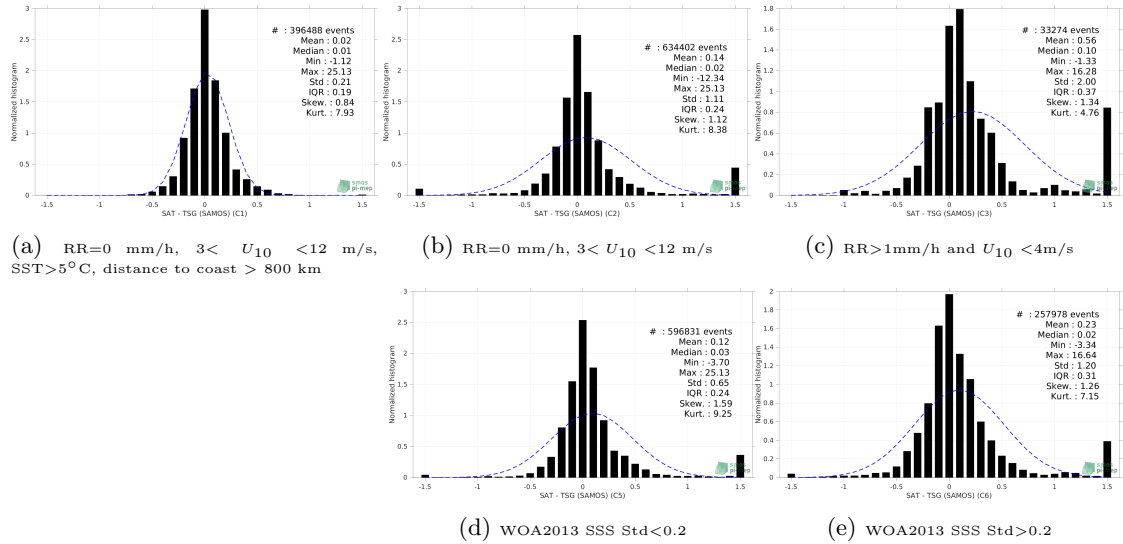
Figure 13: Normalized histogram of \Delta SSS (SMOS SSS L4 v1 - Monthly (CMEMS-CNR) - TSG (SAMOS)) for 5 different subdatasets corresponding to: RR=0 mm/h, 3 < U_{10} < 12 m/s, SST >5^\circ C, distance to coast > 800 km (a), RR=0 mm/h, 3 < U_{10} < 12 m/s (b), RR >1 mm/h and U_{10} < 4 m/s (c), WOA2013 SSS Std <0.2 (d), WOA2013 SSS Std >0.2 (e).
