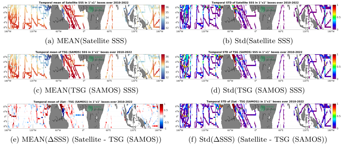
Figure 6: Temporal mean (left) and Std (right) of SSS from SMOS SSS L4 v1 - Monthly (CMEMS-CNR) (top), TSG (SAMOS) (middle), and of \Delta SSS (Satellite - TSG (SAMOS)). Only match-up pairs are used to generate these maps.
