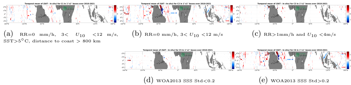
Figure 12: Temporal mean gridded over spatial boxes of size 1^\circ \times 1^\circ of \Delta SSS (SMOS SSS L4 v1 - Monthly (CMEMS-CNR) - TSG (SAMOS)) for 5 different subdatasets corresponding to:RR=0 mm/h, 3 < U_{10} < 12 m/s, SST >5^\circ C, distance to coast > 800 km (a), RR=0 mm/h, 3 < U_{10} < 12 m/s (b), RR >1 mm/h and U_{10} < 4 m/s (c), WOA2013 SSS Std <0.2 (d), WOA2013 SSS Std >0.2 (e).
