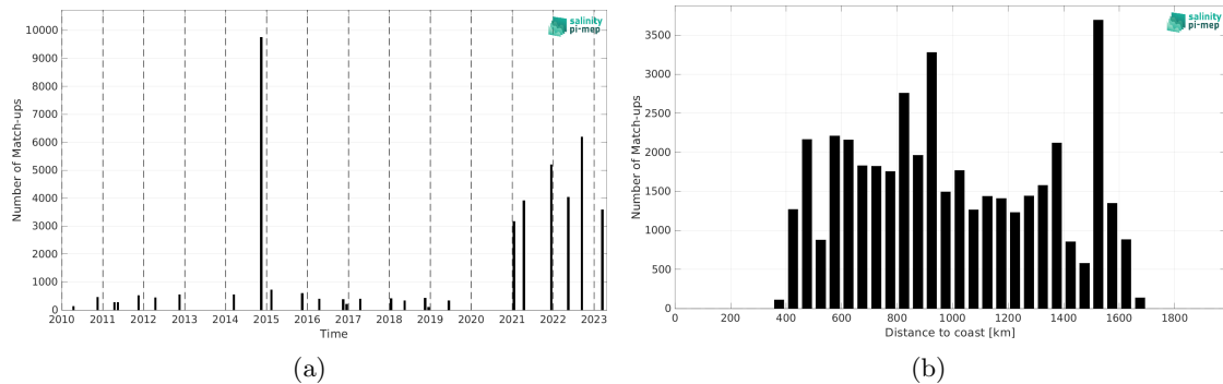
Figure 2: Number of match-ups between TSG (Polarstern) and SMOS SSS L4 v1 - Monthly (CMEMS-CNR) SSS as a function of time (a) and as function of the distance to coast (b) over the Equatorial Ocean 10N-10S Pi-MEP region and for the full satellite product period.
