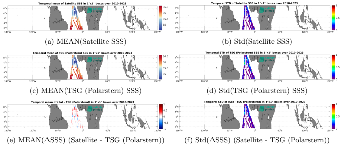
Figure 7: Temporal mean (left) and Std (right) of SSS from SMOS SSS L4 v1 - Monthly (CMEMS-CNR) (top), TSG (Polarstern) (middle), and of \Delta SSS (Satellite - TSG (Polarstern)). Only match-up pairs are used to generate these maps.
