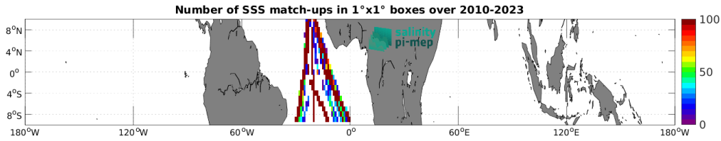
Figure 5: Number of SSS match-ups between TSG (Polarstern) SSS and the SMOS SSS L4 v1 - Monthly (CMEMS-CNR) SSS product for the Equatorial Ocean 10N-10S Pi-MEP region over 1^\circ \times 1^\circ boxes and for the full satellite product period.
