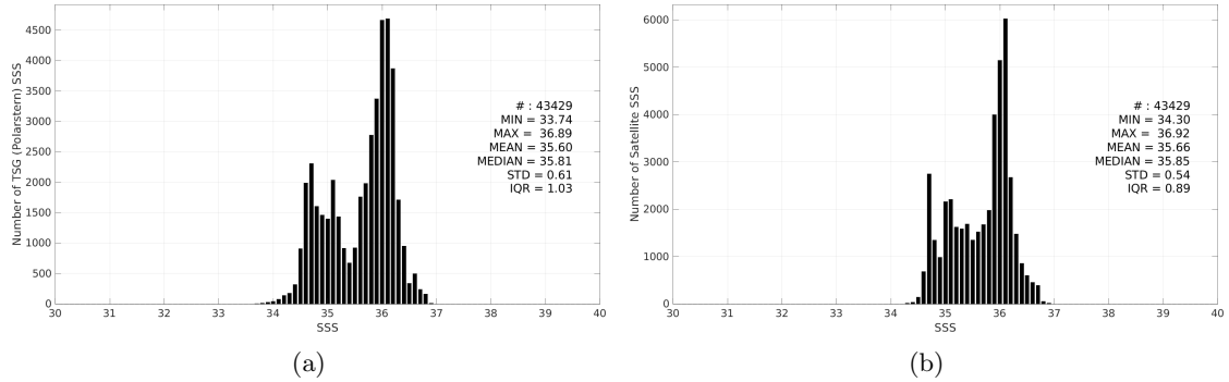
Figure 3: Histograms of SSS from TSG (Polarstern) (a) and SMOS SSS L4 v1 - Monthly (CMEMS-CNR) (b) considering all match-up pairs per bins of 0.1 over the Equatorial Ocean 10N-10S Pi-MEP region and for the full satellite product period.
