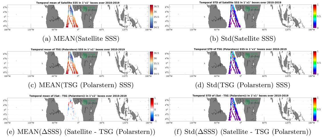
Figure 6: Temporal mean (left) and Std (right) of SSS from SMOS SSS L4 v1 - Monthly (CMEMS-CNR) (top), TSG (Polarstern) (middle), and of \Delta SSS (Satellite - TSG (Polarstern)). Only match-up pairs are used to generate these maps.
