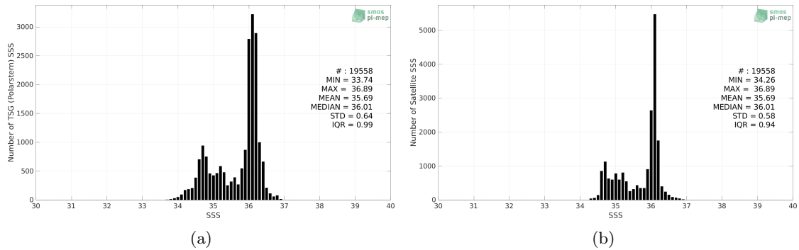
Figure 2: Histograms of SSS from TSG (Polarstern) (a) and SMOS SSS L4 v1 - Monthly (CMEMS-CNR) (b) considering all match-up pairs per bins of 0.1 over the Equatorial Ocean 10N-10S Pi-MEP region and for the full satellite product period.
