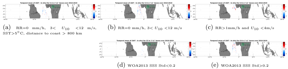
Figure 12: Temporal mean gridded over spatial boxes of size 1^\circ \times 1^\circ of \Delta SSS (SMOS SSS L4 v1 - Monthly (CMEMS-CNR) - TSG (Polarstern)) for 5 different subdatasets corresponding to: RR=0 mm/h, 3 < U_{10} < 12 m/s, SST >5^\circ C, distance to coast > 800 km (a), RR=0 mm/h, 3 < U_{10} < 12 m/s (b), RR >1 mm/h and U_{10} < 4 m/s (c), WOA2013 SSS Std <0.2 (d), WOA2013 SSS Std >0.2 (e).
