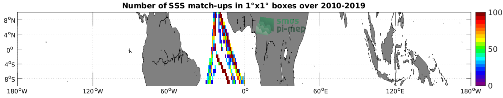
Figure 4: Number of SSS match-ups between TSG (Polarstern) SSS and the SMOS SSS L4 v1 - Monthly (CMEMS-CNR) SSS product for the Equatorial Ocean 10N-10S Pi-MEP region over 1^\circ \times 1^\circ boxes and for the full satellite product period.
