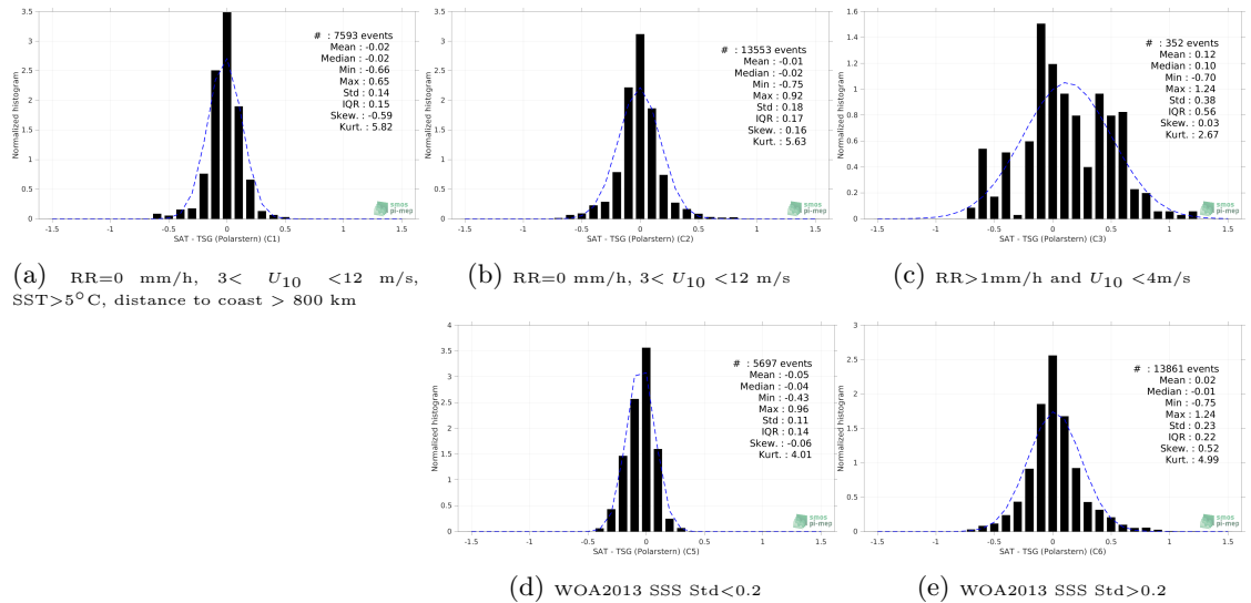
Figure 13: Normalized histogram of \Delta SSS (SMOS SSS L4 v1 - Monthly (CMEMS-CNR) - TSG (Polarstern)) for 5 different subdatasets corresponding to: RR=0 mm/h, 3 < U_{10} < 12 m/s, SST >5^\circ C, distance to coast > 800 km (a), RR=0 mm/h, 3 < U_{10} < 12 m/s (b), RR >1 mm/h and U_{10} < 4 m/s (c), WOA2013 SSS Std <0.2 (d), WOA2013 SSS Std >0.2 (e).
