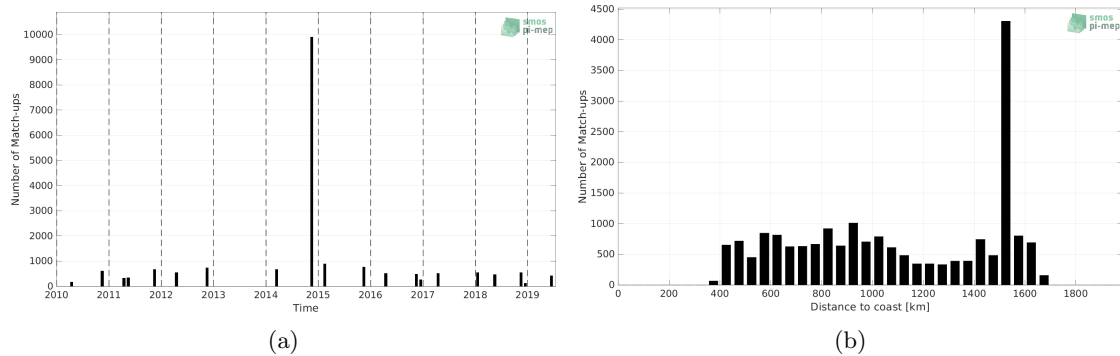
Figure 1: Number of match-ups between TSG (Polarstern) and SMOS SSS L4 v1 - Monthly (CMEMS-CNR) SSS as a function of time (a) and as function of the distance to coast (b) over the Equatorial Ocean 10N-10S Pi-MEP region and for the full satellite product period.
