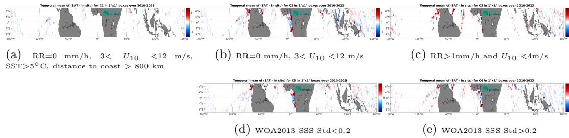
Figure 14: Temporal mean gridded over spatial boxes of size 1^\circ \times 1^\circ of \Delta SSS (SMOS SSS L4 v1 - Monthly (CMEMS-CNR) - TSG (LEGOS-DM)) for 5 different subdatasets corresponding to:RR=0 mm/h, 3 < U_{10} < 12 m/s, SST>5°C, distance to coast > 800 km (a), RR=0 mm/h, 3 < U_{10} < 12 m/s (b), RR>1mm/h and U_{10} < 4 m/s (c), WOA2013 SSS Std<0.2 (d), WOA2013 SSS Std>0.2 (e).
