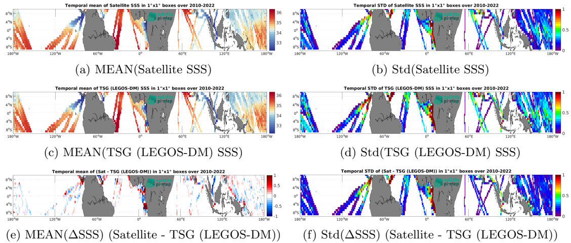
Figure 7: Temporal mean (left) and Std (right) of SSS from SMOS SSS L4 v1 - Monthly (CMEMS-CNR) (top), TSG (LEGOS-DM) (middle), and of \Delta SSS (Satellite - TSG (LEGOS-DM)). Only match-up pairs are used to generate these maps.
