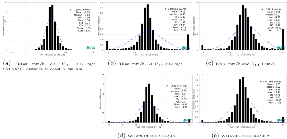
Figure 15: Normalized histogram of \Delta\text{SSS} (SMOS SSS L4 v1 - Monthly (CMEMS-CNR) - TSG (LEGOS-DM)) for 5 different subdatasets corresponding to: RR=0 mm/h, 3 < U_{10} < 12 m/s, SST>5°C, distance to coast > 800 km (a), RR=0 mm/h, 3 < U_{10} < 12 m/s (b), RR>1mm/h and U_{10} < 4 m/s (c), WOA2013 SSS Std<0.2 (d), WOA2013 SSS Std>0.2 (e).
