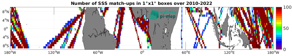
Figure 5: Number of SSS match-ups between TSG (LEGOS-DM) SSS and the SMOS SSS L4 v1 - Monthly (CMEMS-CNR) SSS product for the Equatorial Ocean 10N-10S Pi-MEP region over 1^\circ \times 1^\circ boxes and for the full satellite product period.
