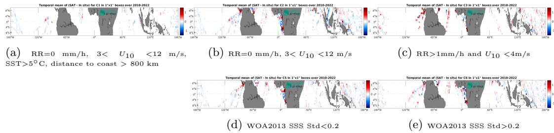
Figure 14: Temporal mean gridded over spatial boxes of size 1^\circ \times 1^\circ of \Delta\text{SSS} (SMOS SSS L4 v1 - Monthly (CMEMS-CNR) - TSG (LEGOS-DM)) for 5 different subdatasets corresponding to:RR=0 mm/h, 3 < U_{10} < 12 m/s, SST>5°C, distance to coast > 800 km (a), RR=0 mm/h, 3 < U_{10} < 12 m/s (b), RR>1mm/h and U_{10} < 4 m/s (c), WOA2013 SSS Std<0.2 (d), WOA2013 SSS Std>0.2 (e).
