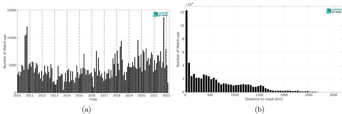
Figure 2: Number of match-ups between TSG (LEGOS-DM) and SMOS SSS L4 v1 - Monthly (CMEMS-CNR) SSS as a function of time (a) and as function of the distance to coast (b) over the Equatorial Ocean 10N-10S Pi-MEP region and for the full satellite product period.
