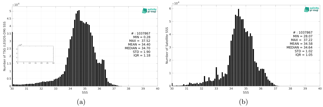
Figure 2: Histograms of SSS from TSG (LEGOS-DM) (a) and SMOS SSS L4 v1 - Monthly (CMEMS-CNR) (b) considering all match-up pairs per bins of 0.1 over the Equatorial Ocean 10N-10S Pi-MEP region and for the full satellite product period.
