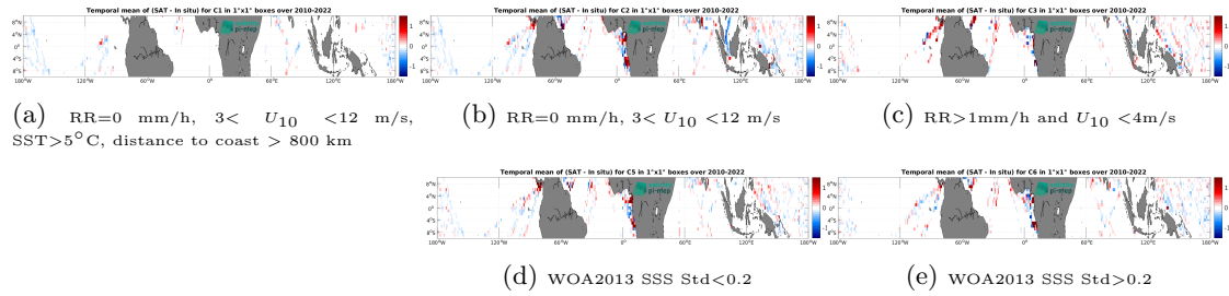
Figure 12: Temporal mean gridded over spatial boxes of size 1^\circ \times 1^\circ of \Delta SSS (SMOS SSS L4 v1 - Monthly (CMEMS-CNR) - TSG (LEGOS-DM)) for 5 different subdatasets corresponding to:RR=0 mm/h, 3 < U_{10} < 12 m/s, SST >5^\circ C, distance to coast > 800 km (a), RR=0 mm/h, 3 < U_{10} < 12 m/s (b), RR >1 mm/h and U_{10} < 4 m/s (c), WOA2013 SSS Std <0.2 (d), WOA2013 SSS Std >0.2 (e).
