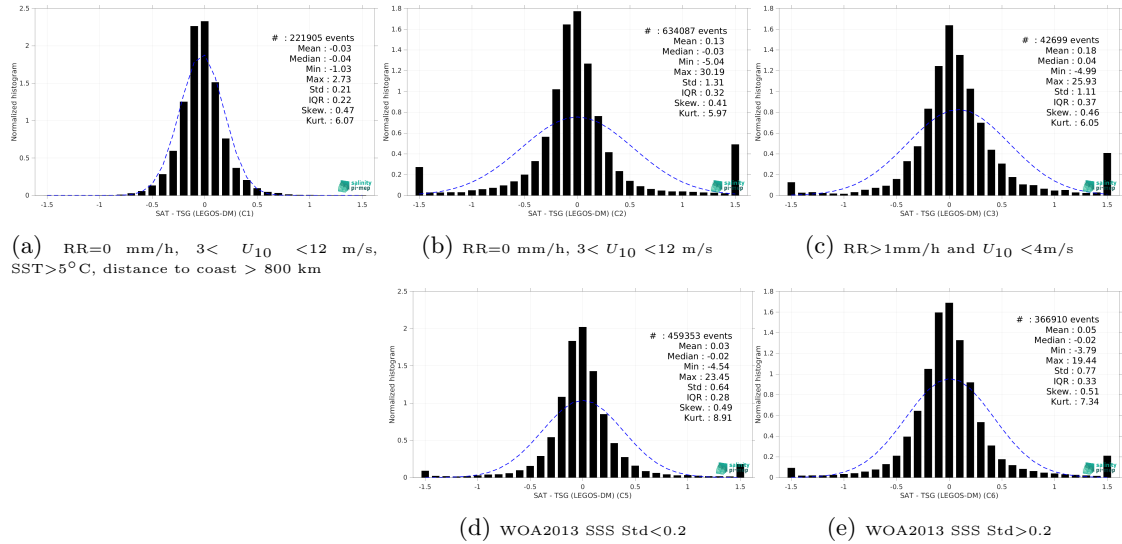
Figure 13: Normalized histogram of \Delta SSS (SMOS SSS L4 v1 - Monthly (CMEMS-CNR) - TSG (LEGOS-DM)) for 5 different subdatasets corresponding to: RR=0 mm/h, 3 < U_{10} < 12 m/s, SST >5^\circ C, distance to coast > 800 km (a), RR=0 mm/h, 3 < U_{10} < 12 m/s (b), RR >1 mm/h and U_{10} < 4 m/s (c), WOA2013 SSS Std <0.2 (d), WOA2013 SSS Std >0.2 (e).
