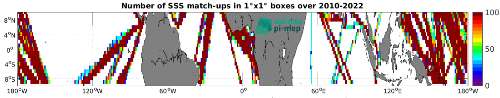
Figure 4: Number of SSS match-ups between TSG (LEGOS-DM) SSS and the SMOS SSS L4 v1 - Monthly (CMEMS-CNR) SSS product for the Equatorial Ocean 10N-10S Pi-MEP region over 1^\circ \times 1^\circ boxes and for the full satellite product period.
