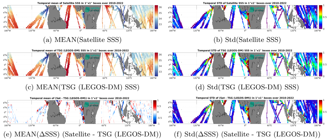
Figure 6: Temporal mean (left) and Std (right) of SSS from SMOS SSS L4 v1 - Monthly (CMEMS-CNR) (top), TSG (LEGOS-DM) (middle), and of \Delta SSS (Satellite - TSG (LEGOS-DM)). Only match-up pairs are used to generate these maps.
