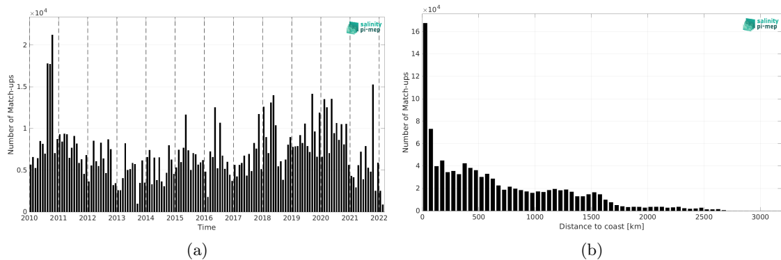
Figure 1: Number of match-ups between TSG (LEGOS-DM) and SMOS SSS L4 v1 - Monthly (CMEMS-CNR) SSS as a function of time (a) and as function of the distance to coast (b) over the Equatorial Ocean 10N-10S Pi-MEP region and for the full satellite product period.
