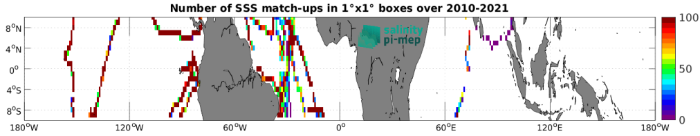
Figure 5: Number of SSS match-ups between TSG (GOSUD-Sailing-ship) SSS and the SMOS SSS L4 v1 - Monthly (CMEMS-CNR) SSS product for the Equatorial Ocean 10N-10S Pi-MEP region over 1^\circ \times 1^\circ boxes and for the full satellite product period.
