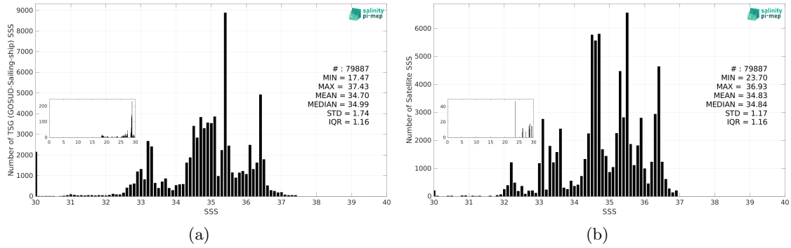
Figure 3: Histograms of SSS from TSG (GOSUD-Sailing-ship) (a) and SMOS SSS L4 v1 - Monthly (CMEMS-CNR) (b) considering all match-up pairs per bins of 0.1 over the Equatorial Ocean 10N-10S Pi-MEP region and for the full satellite product period.
