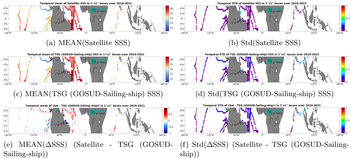
Figure 7: Temporal mean (left) and Std (right) of SSS from SMOS SSS L4 v1 - Monthly (CMEMS-CNR) (top), TSG (GOSUD-Sailing-ship) (middle), and of \Delta SSS (Satellite - TSG (GOSUD-Sailing-ship)). Only match-up pairs are used to generate these maps.
