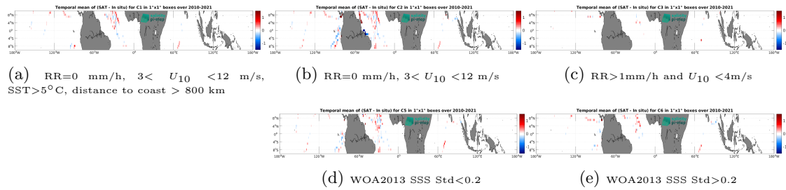
Figure 14: Temporal mean gridded over spatial boxes of size 1^\circ \times 1^\circ of \Delta SSS (SMOS SSS L4 v1 - Monthly (CMEMS-CNR) - TSG (GOSUD-Sailing-ship)) for 5 different subdatasets corresponding to: RR=0 mm/h, 3 < U_{10} < 12 m/s, SST>5°C, distance to coast > 800 km (a), RR=0 mm/h, 3 < U_{10} < 12 m/s (b), RR>1mm/h and U_{10} < 4 m/s (c), WOA2013 SSS Std<0.2 (d), WOA2013 SSS Std>0.2 (e).
