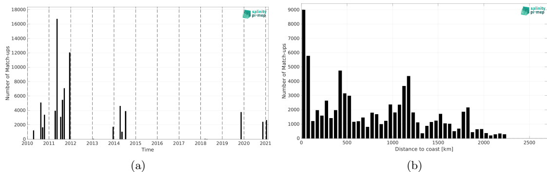
Figure 2: Number of match-ups between TSG (GOSUD-Sailing-ship) and SMOS SSS L4 v1 - Monthly (CMEMS-CNR) SSS as a function of time (a) and as function of the distance to coast (b) over the Equatorial Ocean 10N-10S Pi-MEP region and for the full satellite product period.
