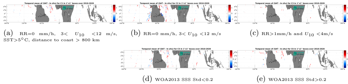
Figure 14: Temporal mean gridded over spatial boxes of size 1^\circ \times 1^\circ of \Delta\text{SSS} (SMOS SSS L4 v1 - Monthly (CMEMS-CNR) - TSG (GOSUD-Sailing-ship)) for 5 different subdatasets corresponding to: RR=0 mm/h, 3 < U_{10} < 12 m/s, SST>5°C, distance to coast > 800 km (a), RR=0 mm/h, 3 < U_{10} < 12 m/s (b), RR>1mm/h and U_{10} < 4 m/s (c), WOA2013 SSS Std<0.2 (d), WOA2013 SSS Std>0.2 (e).
