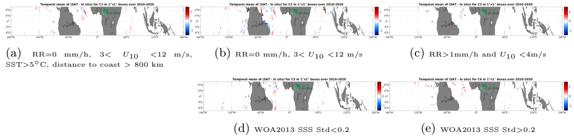
Figure 12: Temporal mean gridded over spatial boxes of size 1^\circ \times 1^\circ of \Delta\text{SSS} (SMOS SSS L4 v1 - Monthly (CMEMS-CNR) - TSG (GOSUD-Sailing-ship)) for 5 different subdatasets corresponding to: RR=0 mm/h, 3 < U_{10} < 12 m/s, SST>5°C, distance to coast > 800 km (a), RR=0 mm/h, 3 < U_{10} < 12 m/s (b), RR>1mm/h and U_{10} < 4 m/s (c), WOA2013 SSS Std<0.2 (d), WOA2013 SSS Std>0.2 (e).
