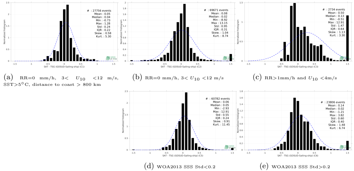
Figure 13: Normalized histogram of \Delta\text{SSS} (SMOS SSS L4 v1 - Monthly (CMEMS-CNR) - TSG (GOSUD-Sailing-ship)) for 5 different subdatasets corresponding to: RR=0 mm/h, 3 < U_{10} < 12 m/s, SST>5°C, distance to coast > 800 km (a), RR=0 mm/h, 3 < U_{10} < 12 m/s (b), RR>1mm/h and U_{10} < 4 m/s (c), WOA2013 SSS Std<0.2 (d), WOA2013 SSS Std>0.2 (e).
