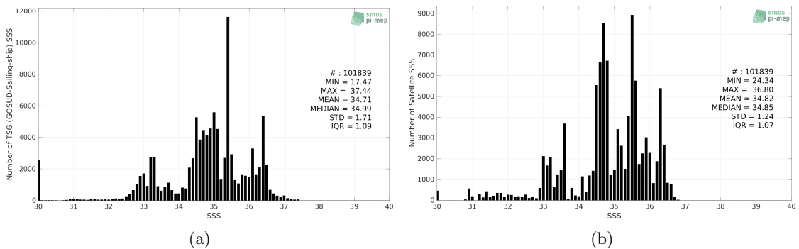
Figure 2: Histograms of SSS from TSG (GOSUD-Sailing-ship) (a) and SMOS SSS L4 v1 - Monthly (CMEMS-CNR) (b) considering all match-up pairs per bins of 0.1 over the Equatorial Ocean 10N-10S Pi-MEP region and for the full satellite product period.
