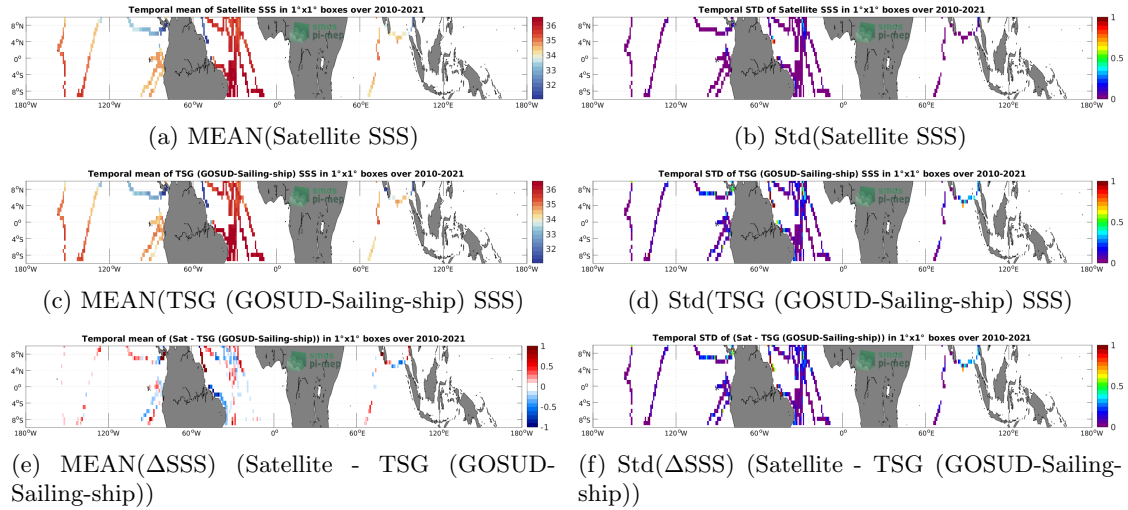
Figure 6: Temporal mean (left) and Std (right) of SSS from SMOS SSS L4 v1 - Monthly (CMEMS-CNR) (top), TSG (GOSUD-Sailing-ship) (middle), and of \Delta SSS (Satellite - TSG (GOSUD-Sailing-ship)). Only match-up pairs are used to generate these maps.
