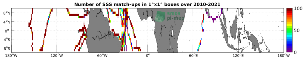
Figure 4: Number of SSS match-ups between TSG (GOSUD-Sailing-ship) SSS and the SMOS SSS L4 v1 - Monthly (CMEMS-CNR) SSS product for the Equatorial Ocean 10N-10S Pi-MEP region over 1^\circ \times 1^\circ boxes and for the full satellite product period.
