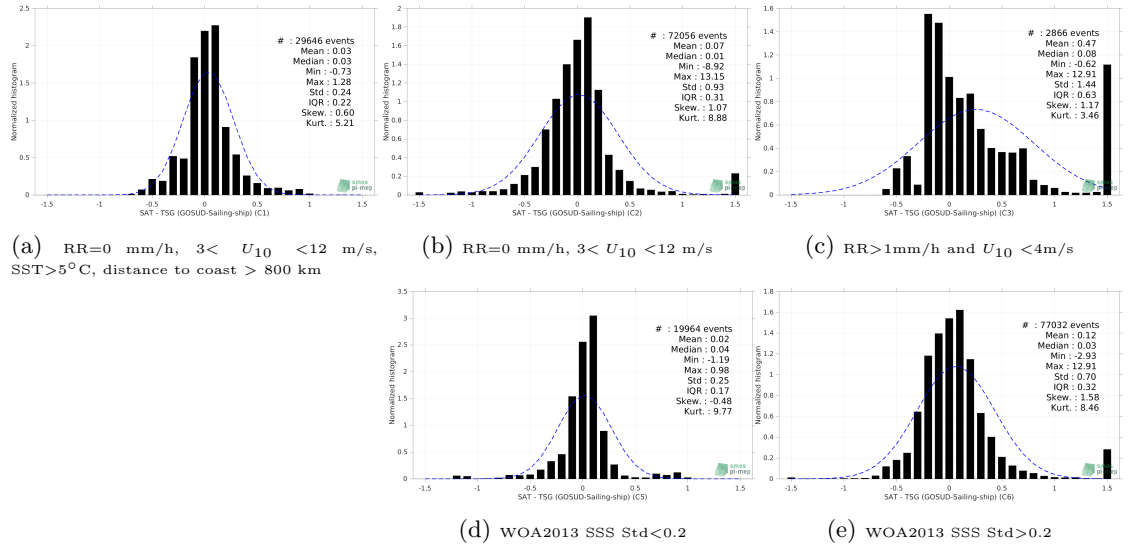
Figure 13: Normalized histogram of \Delta SSS (SMOS SSS L4 v1 - Monthly (CMEMS-CNR) - TSG (GOSUD-Sailing-ship)) for 5 different subdatasets corresponding to: RR=0 mm/h, 3 < U_{10} < 12 m/s, SST >5^\circ C, distance to coast > 800 km (a), RR=0 mm/h, 3 < U_{10} < 12 m/s (b), RR >1 mm/h and U_{10} < 4 m/s (c), WOA2013 SSS Std <0.2 (d), WOA2013 SSS Std >0.2 (e).
