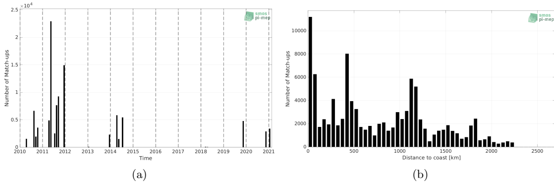
Figure 1: Number of match-ups between TSG (GOSUD-Sailing-ship) and SMOS SSS L4 v1 - Monthly (CMEMS-CNR) SSS as a function of time (a) and as function of the distance to coast (b) over the Equatorial Ocean 10N-10S Pi-MEP region and for the full satellite product period.
