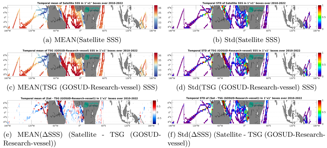
Figure 7: Temporal mean (left) and Std (right) of SSS from SMOS SSS L4 v1 - Monthly (CMEMS-CNR) (top), TSG (GOSUD-Research-vessel) (middle), and of \Delta SSS (Satellite - TSG (GOSUD-Research-vessel)). Only match-up pairs are used to generate these maps.
