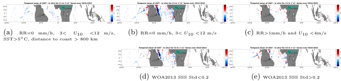
Figure 14: Temporal mean gridded over spatial boxes of size 1^\circ \times 1^\circ of \Delta\text{SSS} (SMOS SSS L4 v1 - Monthly (CMEMS-CNR) - TSG (GOSUD-Research-vessel)) for 5 different subdatasets corresponding to: RR=0 mm/h, 3 < U_{10} < 12 m/s, SST>5°C, distance to coast > 800 km (a), RR=0 mm/h, 3 < U_{10} < 12 m/s (b), RR>1mm/h and U_{10} < 4 m/s (c), WOA2013 SSS Std<0.2 (d), WOA2013 SSS Std>0.2 (e).
