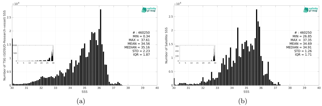
Figure 3: Histograms of SSS from TSG (GOSUD-Research-vessel) (a) and SMOS SSS L4 v1 - Monthly (CMEMS-CNR) (b) considering all match-up pairs per bins of 0.1 over the Equatorial Ocean 10N-10S Pi-MEP region and for the full satellite product period.
