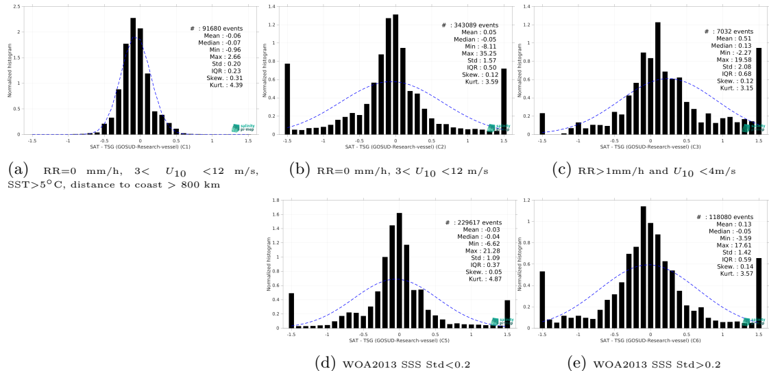
Figure 15: Normalized histogram of \Delta\text{SSS} (SMOS SSS L4 v1 - Monthly (CMEMS-CNR) - TSG (GOSUD-Research-vessel)) for 5 different subdatasets corresponding to: RR=0 mm/h, 3 < U_{10} < 12 m/s, SST>5°C, distance to coast > 800 km (a), RR=0 mm/h, 3 < U_{10} < 12 m/s (b), RR>1mm/h and U_{10} < 4 m/s (c), WOA2013 SSS Std<0.2 (d), WOA2013 SSS Std>0.2 (e).
