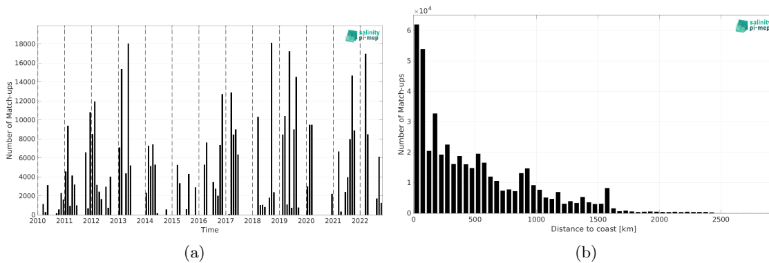
Figure 2: Number of match-ups between TSG (GOSUD-Research-vessel) and SMOS SSS L4 v1 - Monthly (CMEMS-CNR) SSS as a function of time (a) and as function of the distance to coast (b) over the Equatorial Ocean 10N-10S Pi-MEP region and for the full satellite product period.
