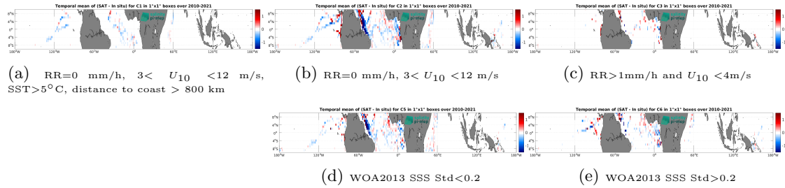
Figure 14: Temporal mean gridded over spatial boxes of size 1^\circ \times 1^\circ of \Delta SSS (SMOS SSS L4 v1 - Monthly (CMEMS-CNR) - TSG (GOSUD-Research-vessel)) for 5 different subdatasets corresponding to:RR=0 mm/h, 3 < U_{10} < 12 m/s, SST>5°C, distance to coast > 800 km (a), RR=0 mm/h, 3 < U_{10} < 12 m/s (b), RR>1mm/h and U_{10} < 4 m/s (c), WOA2013 SSS Std<0.2 (d), WOA2013 SSS Std>0.2 (e).
