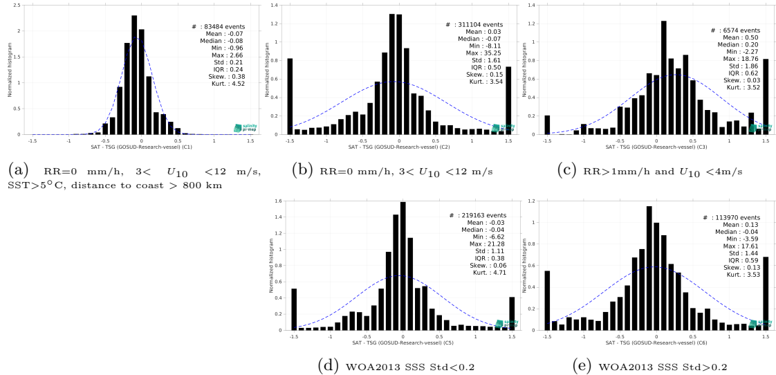
Figure 15: Normalized histogram of \Delta SSS (SMOS SSS L4 v1 - Monthly (CMEMS-CNR) - TSG (GOSUD-Research-vessel)) for 5 different subdatasets corresponding to: RR=0 mm/h, 3 < U_{10} < 12 m/s, SST>5°C, distance to coast > 800 km (a), RR=0 mm/h, 3 < U_{10} < 12 m/s (b), RR>1mm/h and U_{10} < 4 m/s (c), WOA2013 SSS Std<0.2 (d), WOA2013 SSS Std>0.2 (e).
