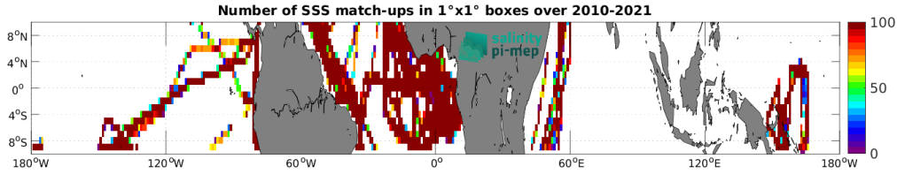
Figure 4: Number of SSS match-ups between TSG (GOSUD-Research-vessel) SSS and the SMOS SSS L4 v1 - Monthly (CMEMS-CNR) SSS product for the Equatorial Ocean 10N-10S Pi-MEP region over 1^\circ \times 1^\circ boxes and for the full satellite product period.
