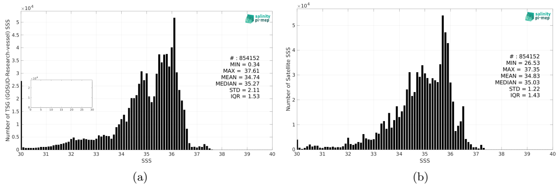
Figure 2: Histograms of SSS from TSG (GOSUD-Research-vessel) (a) and SMOS SSS L4 v1 - Monthly (CMEMS-CNR) (b) considering all match-up pairs per bins of 0.1 over the Equatorial Ocean 10N-10S Pi-MEP region and for the full satellite product period.
