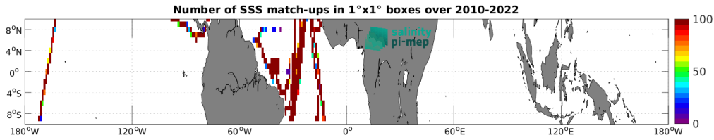
Figure 5: Number of SSS match-ups between TSG (CSIC-UTM) SSS and the SMOS SSS L4 v1 - Monthly (CMEMS-CNR) SSS product for the Equatorial Ocean 10N-10S Pi-MEP region over 1^\circ \times 1^\circ boxes and for the full satellite product period.
