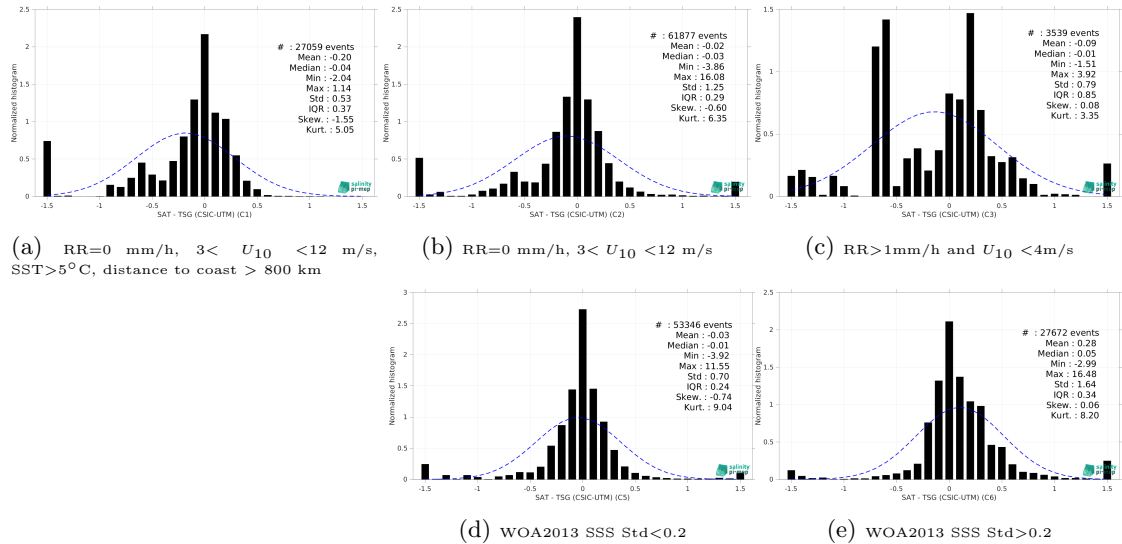
Figure 15: Normalized histogram of \Delta\text{SSS} (SMOS SSS L4 v1 - Monthly (CMEMS-CNR) - TSG (CSIC-UTM)) for 5 different subdatasets corresponding to: RR=0 mm/h, 3 < U_{10} < 12 m/s, SST>5°C, distance to coast > 800 km (a), RR=0 mm/h, 3 < U_{10} < 12 m/s (b), RR>1mm/h and U_{10} < 4 m/s (c), WOA2013 SSS Std<0.2 (d), WOA2013 SSS Std>0.2 (e).
