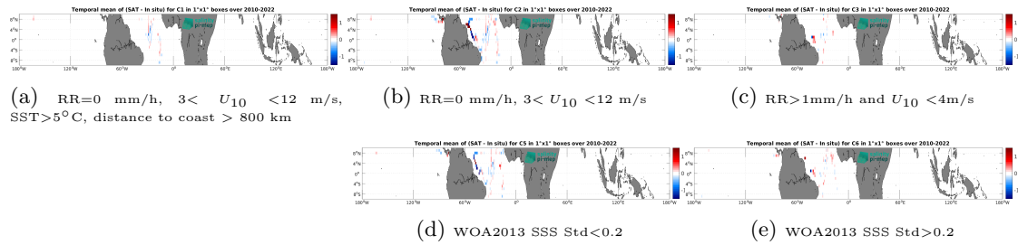
Figure 14: Temporal mean gridded over spatial boxes of size 1^\circ \times 1^\circ of \Delta\text{SSS} (SMOS SSS L4 v1 - Monthly (CMEMS-CNR) - TSG (CSIC-UTM)) for 5 different subdatasets corresponding to:RR=0 mm/h, 3 < U_{10} < 12 m/s, SST>5°C, distance to coast > 800 km (a), RR=0 mm/h, 3 < U_{10} < 12 m/s (b), RR>1mm/h and U_{10} < 4 m/s (c), WOA2013 SSS Std<0.2 (d), WOA2013 SSS Std>0.2 (e).
