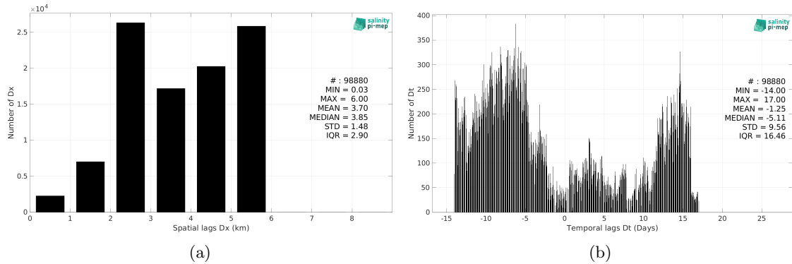
Figure 6: Histograms of the spatial (a) and temporal (b) lags between the location/time of the TSG (CSIC-UTM) measurement and the date of the corresponding SMOS SSS L4 v1 - Monthly (CMEMS-CNR) SSS pixel.
