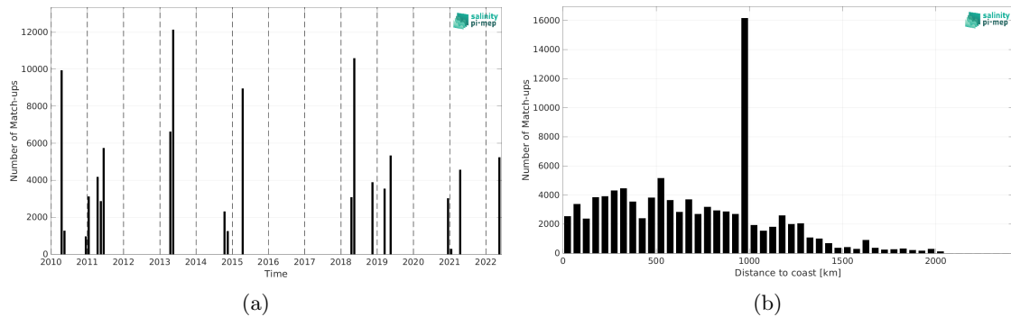
Figure 2: Number of match-ups between TSG (CSIC-UTM) and SMOS SSS L4 v1 - Monthly (CMEMS-CNR) SSS as a function of time (a) and as function of the distance to coast (b) over the Equatorial Ocean 10N-10S Pi-MEP region and for the full satellite product period.
