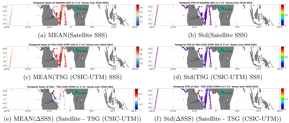
Figure 7: Temporal mean (left) and Std (right) of SSS from SMOS SSS L4 v1 - Monthly (CMEMS-CNR) (top), TSG (CSIC-UTM) (middle), and of \Delta SSS (Satellite - TSG (CSIC-UTM)). Only match-up pairs are used to generate these maps.
