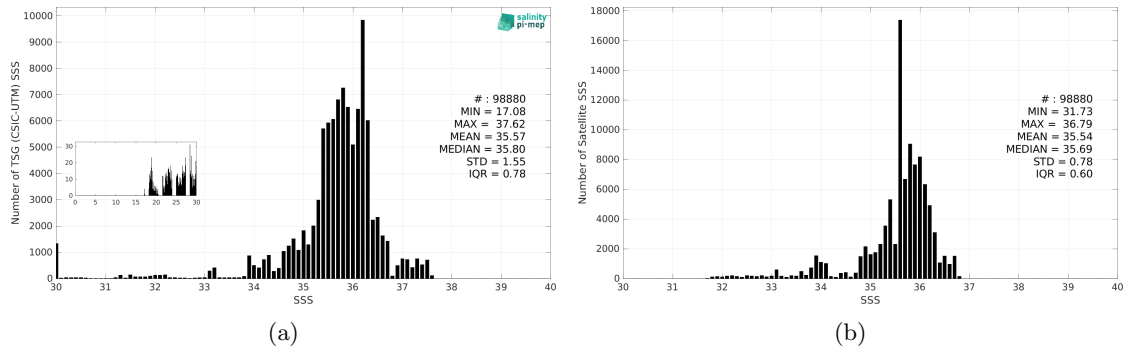
Figure 3: Histograms of SSS from TSG (CSIC-UTM) (a) and SMOS SSS L4 v1 - Monthly (CMEMS-CNR) (b) considering all match-up pairs per bins of 0.1 over the Equatorial Ocean 10N-10S Pi-MEP region and for the full satellite product period.
