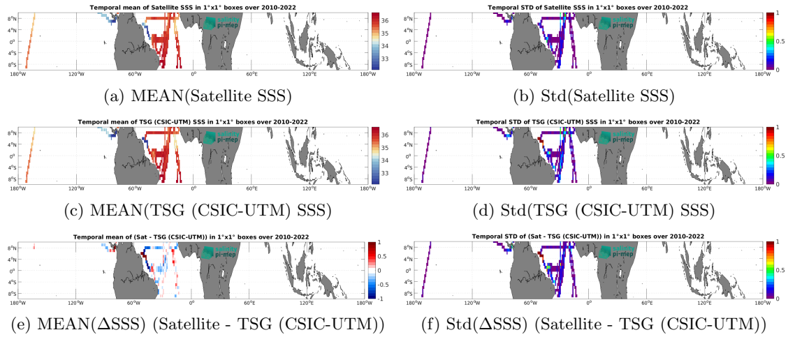
Figure 6: Temporal mean (left) and Std (right) of SSS from SMOS SSS L4 v1 - Monthly (CMEMS-CNR) (top), TSG (CSIC-UTM) (middle), and of \Delta SSS (Satellite - TSG (CSIC-UTM)). Only match-up pairs are used to generate these maps.
