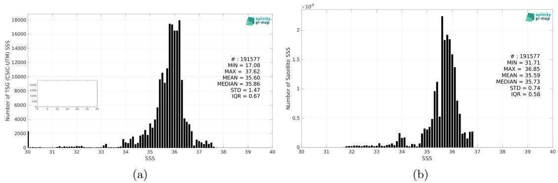
Figure 2: Histograms of SSS from TSG (CSIC-UTM) (a) and SMOS SSS L4 v1 - Monthly (CMEMS-CNR) (b) considering all match-up pairs per bins of 0.1 over the Equatorial Ocean 10N-10S Pi-MEP region and for the full satellite product period.
