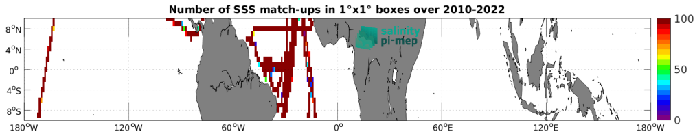
Figure 4: Number of SSS match-ups between TSG (CSIC-UTM) SSS and the SMOS SSS L4 v1 - Monthly (CMEMS-CNR) SSS product for the Equatorial Ocean 10N-10S Pi-MEP region over 1^\circ \times 1^\circ boxes and for the full satellite product period.
