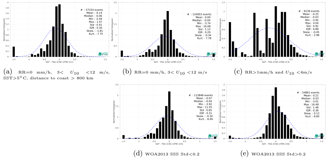
Figure 13: Normalized histogram of \Delta SSS (SMOS SSS L4 v1 - Monthly (CMEMS-CNR) - TSG (CSIC-UTM)) for 5 different subdatasets corresponding to: RR=0 mm/h, 3 < U_{10} < 12 m/s, SST >5^\circ C, distance to coast > 800 km (a), RR=0 mm/h, 3 < U_{10} < 12 m/s (b), RR >1 mm/h and U_{10} < 4 m/s (c), WOA2013 SSS Std <0.2 (d), WOA2013 SSS Std >0.2 (e).
