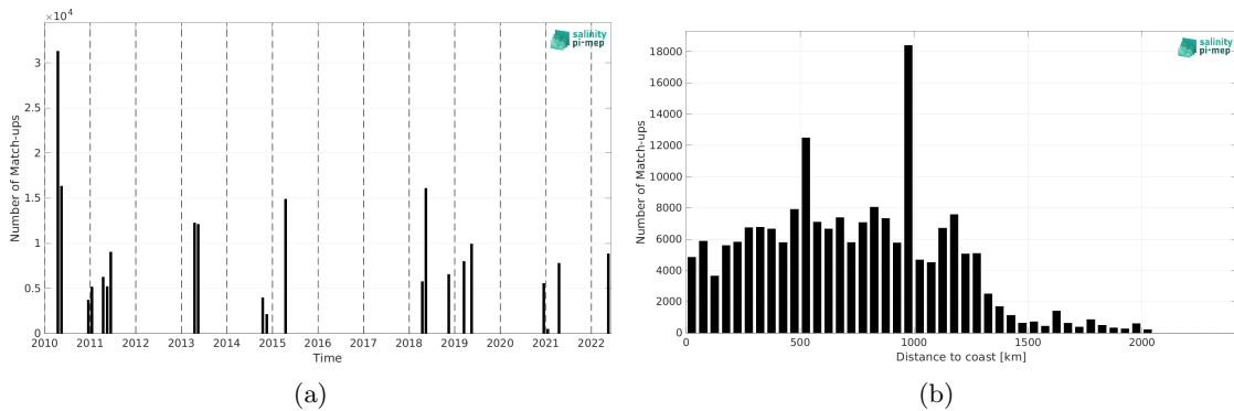
Figure 1: Number of match-ups between TSG (CSIC-UTM) and SMOS SSS L4 v1 - Monthly (CMEMS-CNR) SSS as a function of time (a) and as function of the distance to coast (b) over the Equatorial Ocean 10N-10S Pi-MEP region and for the full satellite product period.
