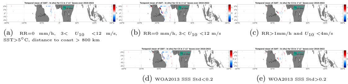
Figure 12: Temporal mean gridded over spatial boxes of size 1^\circ \times 1^\circ of \Delta SSS (SMOS SSS L4 v1 - Monthly (CMEMS-CNR) - TSG (CSIC-UTM)) for 5 different subdatasets corresponding to:RR=0 mm/h, 3 < U_{10} < 12 m/s, SST >5^\circ C, distance to coast > 800 km (a), RR=0 mm/h, 3 < U_{10} < 12 m/s (b), RR >1 mm/h and U_{10} < 4 m/s (c), WOA2013 SSS Std <0.2 (d), WOA2013 SSS Std >0.2 (e).
