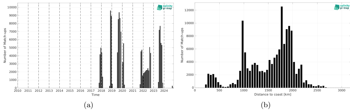
Figure 2: Number of match-ups between Saildrone and SMOS SSS L4 v1 - Monthly (CMEMS-CNR) SSS as a function of time (a) and as function of the distance to coast (b) over the Equatorial Ocean 10N-10S Pi-MEP region and for the full satellite product period.
