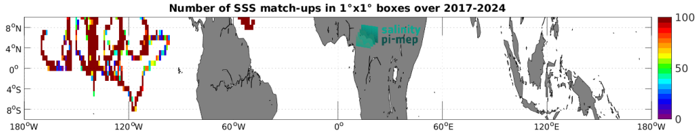
Figure 5: Number of SSS match-ups between Saildrone SSS and the SMOS SSS L4 v1 - Monthly (CMEMS-CNR) SSS product for the Equatorial Ocean 10N-10S Pi-MEP region over 1^\circ \times 1^\circ boxes and for the full satellite product period.
