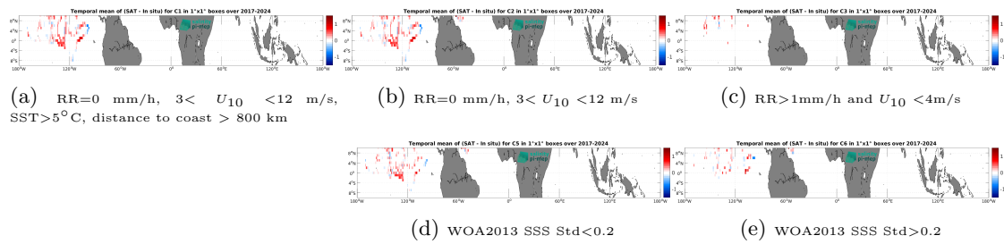
Figure 14: Temporal mean gridded over spatial boxes of size 1^\circ \times 1^\circ of \Delta SSS (SMOS SSS L4 v1 - Monthly (CMEMS-CNR) - Saildrone) for 5 different subdatasets corresponding to:RR=0 mm/h, 3 < U_{10} < 12 m/s, SST>5°C, distance to coast > 800 km (a), RR=0 mm/h, 3 < U_{10} < 12 m/s (b), RR>1mm/h and U_{10} < 4 m/s (c), WOA2013 SSS Std<0.2 (d), WOA2013 SSS Std>0.2 (e).
