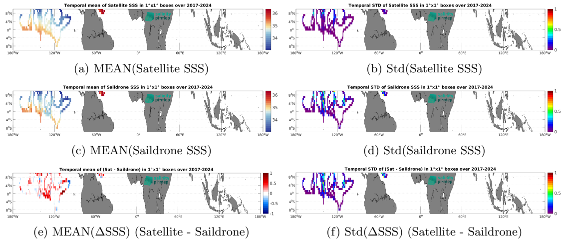
Figure 7: Temporal mean (left) and Std (right) of SSS from SMOS SSS L4 v1 - Monthly (CMEMS-CNR) (top), Saildrone (middle), and of \Delta SSS (Satellite - Saildrone). Only match-up pairs are used to generate these maps.
