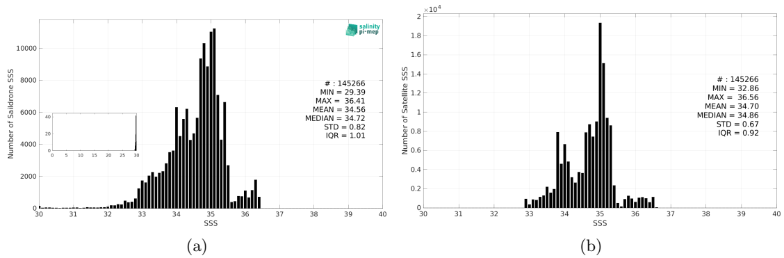
Figure 3: Histograms of SSS from Saildrone (a) and SMOS SSS L4 v1 - Monthly (CMEMS-CNR) (b) considering all match-up pairs per bins of 0.1 over the Equatorial Ocean 10N-10S Pi-MEP region and for the full satellite product period.
