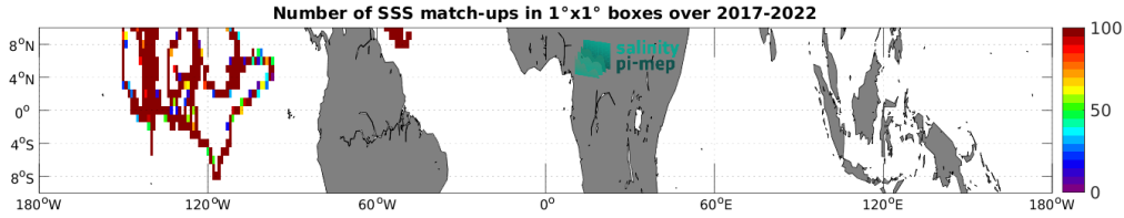
Figure 4: Number of SSS match-ups between Saildrone SSS and the SMOS SSS L4 v1 - Monthly (CMEMS-CNR) SSS product for the Equatorial Ocean 10N-10S Pi-MEP region over 1^\circ \times 1^\circ boxes and for the full satellite product period.
