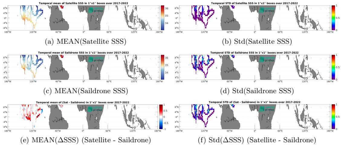
Figure 6: Temporal mean (left) and Std (right) of SSS from SMOS SSS L4 v1 - Monthly (CMEMS-CNR) (top), Saildrone (middle), and of \Delta SSS (Satellite - Saildrone). Only match-up pairs are used to generate these maps.
