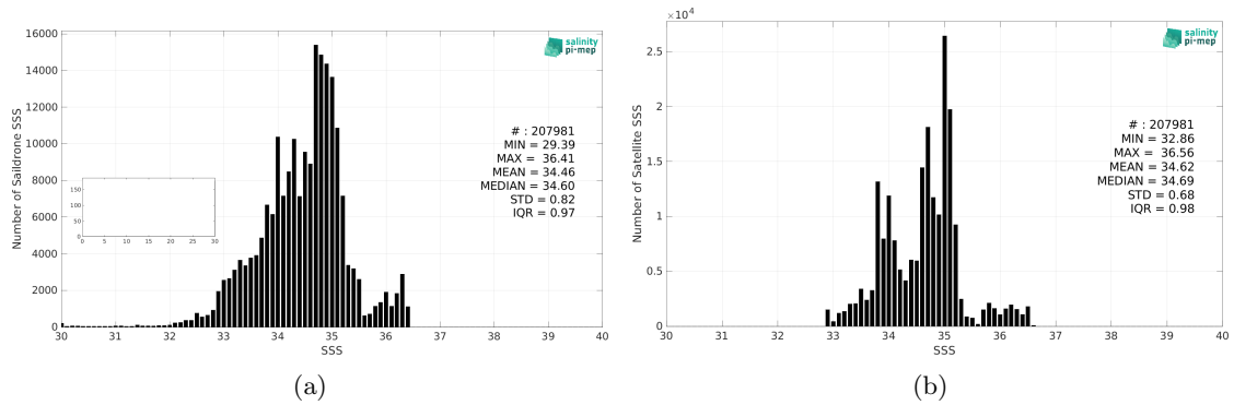
Figure 2: Histograms of SSS from Saildrone (a) and SMOS SSS L4 v1 - Monthly (CMEMS-CNR) (b) considering all match-up pairs per bins of 0.1 over the Equatorial Ocean 10N-10S Pi-MEP region and for the full satellite product period.
