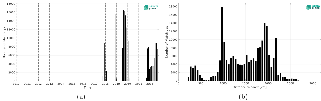
Figure 1: Number of match-ups between Saildrone and SMOS SSS L4 v1 - Monthly (CMEMS-CNR) SSS as a function of time (a) and as function of the distance to coast (b) over the Equatorial Ocean 10N-10S Pi-MEP region and for the full satellite product period.
