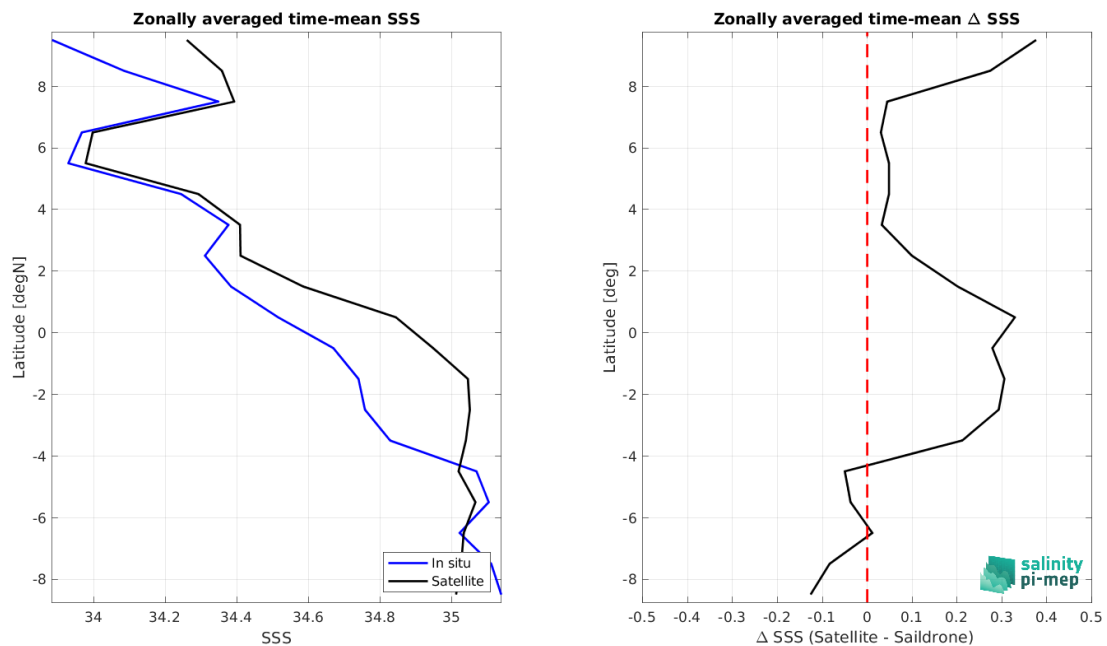
Figure 8: Left panel: Zonal mean SSS from SMOS SSS L4 v1 - Monthly (CMEMS-CNR) satellite product (black) and from Sairdrone (blue). Right panel: Zonal mean of \Delta SSS (Satellite - Sairdrone) for all the collected Pi-MEP match-up pairs estimated over the full satellite product period.
