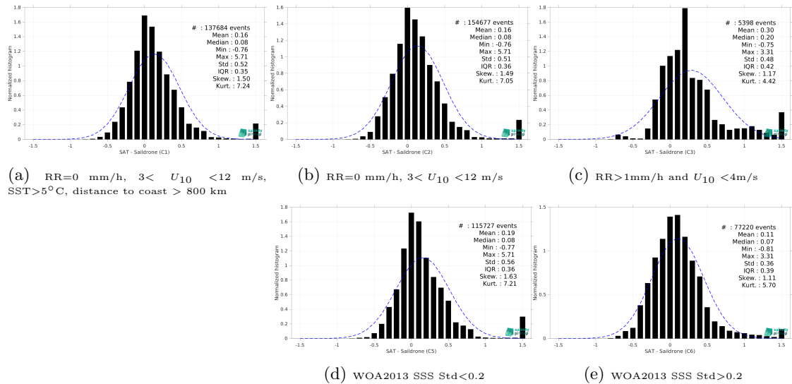
Figure 13: Normalized histogram of \Delta SSS (SMOS SSS L4 v1 - Monthly (CMEMS-CNR) - Saildrone) for 5 different subdatasets corresponding to: RR=0 mm/h, 3 < U_{10} < 12 m/s, SST >5^\circ\text{C} , distance to coast > 800 km (a), RR=0 mm/h, 3 < U_{10} < 12 m/s (b), RR >1 mm/h and U_{10} < 4 m/s (c), WOA2013 SSS Std <0.2 (d), WOA2013 SSS Std >0.2 (e).
