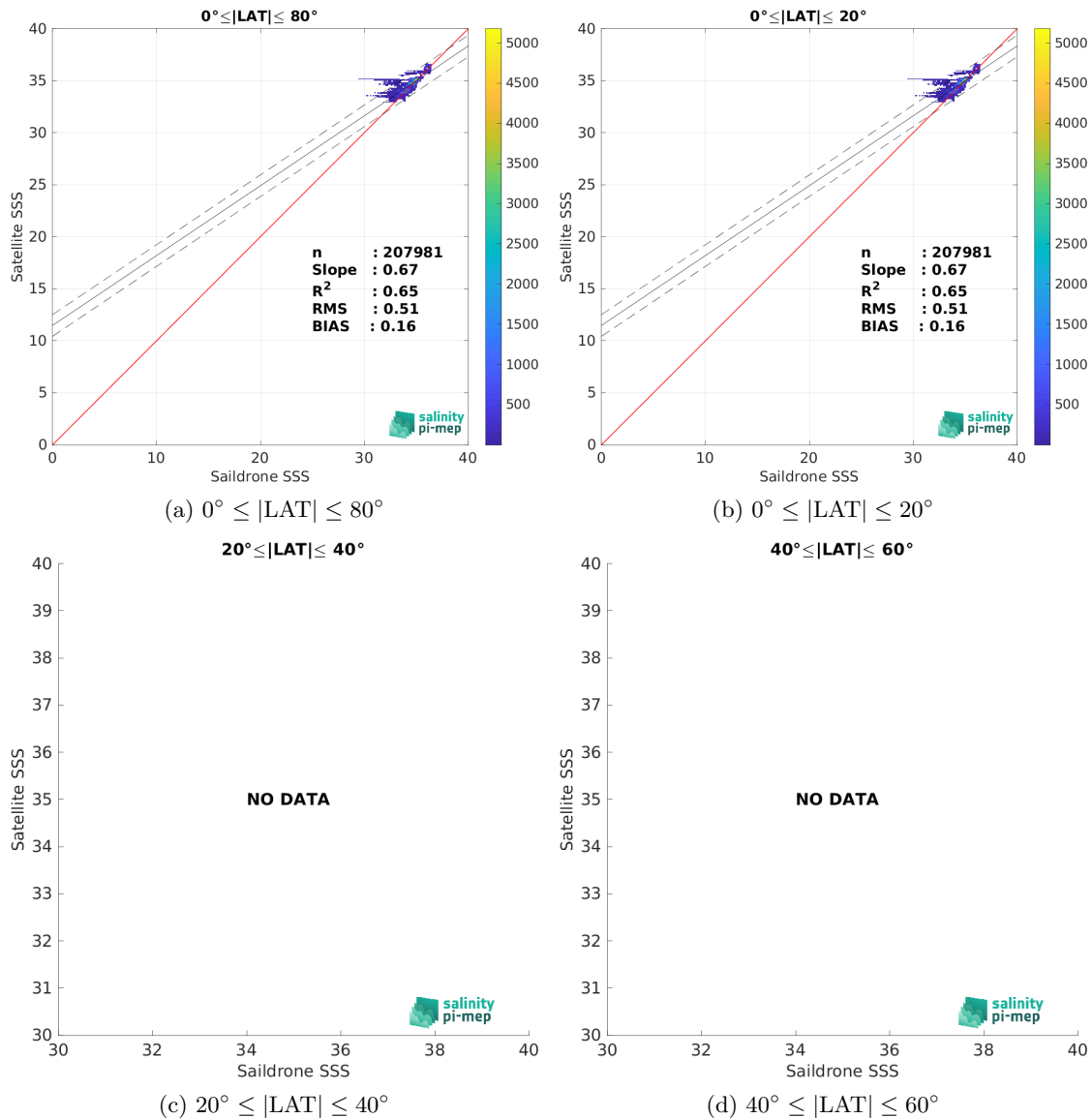
Figure 9: Contour maps of the concentration of SMOS SSS L4 v1 - Monthly (CMEMS-CNR) SSS (y-axis) versus Saildrone SSS (x-axis) at match-up pairs for different latitude bands. For each plot, the red line shows x=y . The black thin and dashed lines indicate a linear fit through the data cloud and the \pm 95\% confidence levels, respectively. The number match-up pairs n , the slope and R^2 coefficient of the linear fit, the root mean square (RMS) and the mean bias between satellite and in situ data are indicated for each latitude band in each plots.
