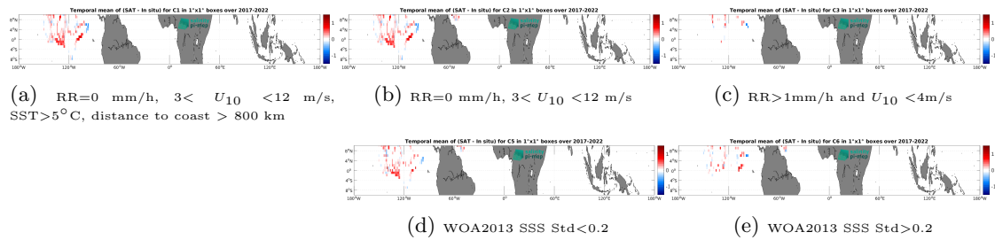
Figure 12: Temporal mean gridded over spatial boxes of size 1^\circ \times 1^\circ of \Delta SSS (SMOS SSS L4 v1 - Monthly (CMEMS-CNR) - Saildrone) for 5 different subdatasets corresponding to: RR=0 mm/h, 3 < U_{10} < 12 m/s, SST >5^\circ\text{C} , distance to coast > 800 km (a), RR=0 mm/h, 3 < U_{10} < 12 m/s (b), RR >1 mm/h and U_{10} < 4 m/s (c), WOA2013 SSS Std <0.2 (d), WOA2013 SSS Std >0.2 (e).
