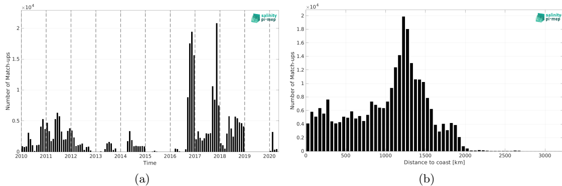
Figure 2: Number of match-ups between Surface drifters and SMOS SSS L4 v1 - Monthly (CMEMS-CNR) SSS as a function of time (a) and as function of the distance to coast (b) over the Equatorial Ocean 10N-10S Pi-MEP region and for the full satellite product period.
