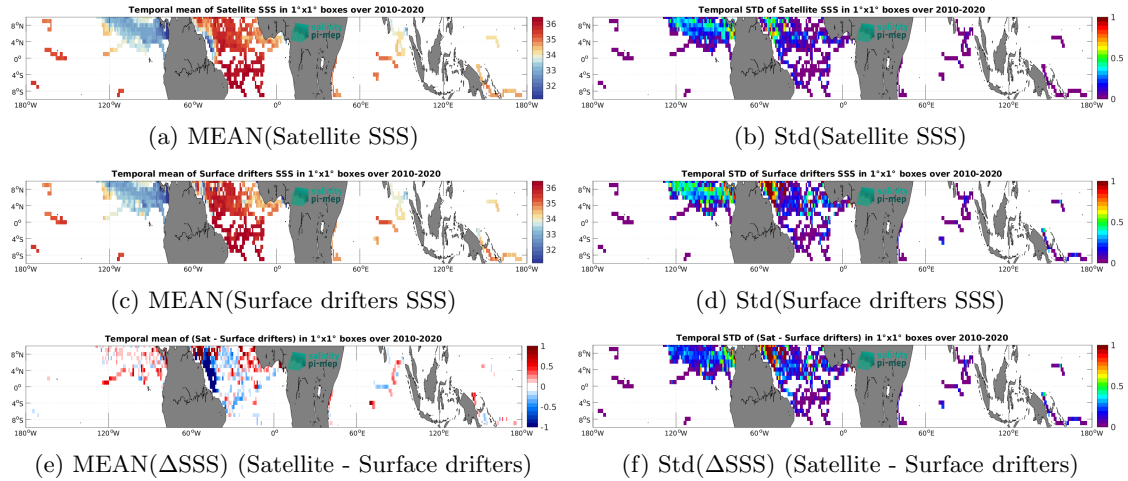
Figure 6: Temporal mean (left) and Std (right) of SSS from SMOS SSS L4 v1 - Monthly (CMEMS-CNR) (top), Surface drifters (middle), and of \Delta SSS (Satellite - Surface drifters). Only match-up pairs are used to generate these maps.
