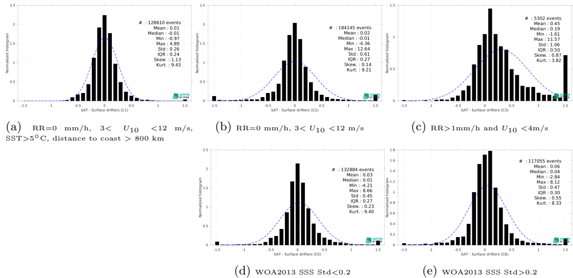
Figure 14: Normalized histogram of \Delta SSS (SMOS SSS L4 v1 - Monthly (CMEMS-CNR) - Surface drifters) for 5 different subdatasets corresponding to: RR=0 mm/h, 3 < U_{10} < 12 m/s, SST >5^\circ C, distance to coast > 800 km (a), RR=0 mm/h, 3 < U_{10} < 12 m/s (b), RR >1 mm/h and U_{10} < 4 m/s (c), WOA2013 SSS Std <0.2 (d), WOA2013 SSS Std >0.2 (e).
