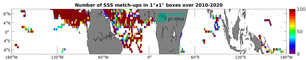
Figure 4: Number of SSS match-ups between Surface drifters SSS and the SMOS SSS L4 v1 - Monthly (CMEMS-CNR) SSS product for the Equatorial Ocean 10N-10S Pi-MEP region over 1^\circ \times 1^\circ boxes and for the full satellite product period.
