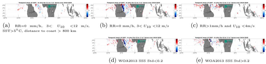
Figure 13: Temporal mean gridded over spatial boxes of size 1^\circ \times 1^\circ of \Delta SSS (SMOS SSS L4 v1 - Monthly (CMEMS-CNR) - Surface drifters) for 5 different subdatasets corresponding to: RR=0 mm/h, 3 < U_{10} < 12 m/s, SST >5^\circ C, distance to coast > 800 km (a), RR=0 mm/h, 3 < U_{10} < 12 m/s (b), RR >1 mm/h and U_{10} < 4 m/s (c), WOA2013 SSS Std <0.2 (d), WOA2013 SSS Std >0.2 (e).
