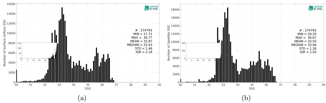
Figure 3: Histograms of SSS from Surface drifters (a) and SMOS SSS L4 v1 - Monthly (CMEMS-CNR) (b) considering all match-up pairs per bins of 0.1 over the Equatorial Ocean 10N-10S Pi-MEP region and for the full satellite product period.
