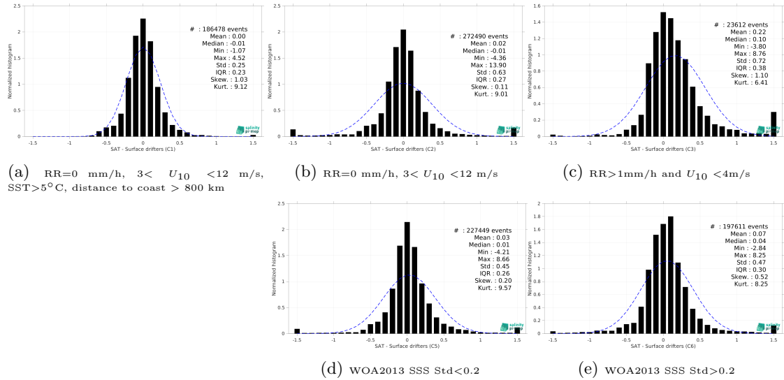
Figure 12: Normalized histogram of \Delta SSS (SMOS SSS L4 v1 - Monthly (CMEMS-CNR) - Surface drifters) for 5 different subdatasets corresponding to: RR=0 mm/h, 3 < U_{10} < 12 m/s, SST >5^\circ\text{C} , distance to coast > 800 km (a), RR=0 mm/h, 3 < U_{10} < 12 m/s (b), RR >1 mm/h and U_{10} < 4 m/s (c), WOA2013 SSS Std <0.2 (d), WOA2013 SSS Std >0.2 (e).
