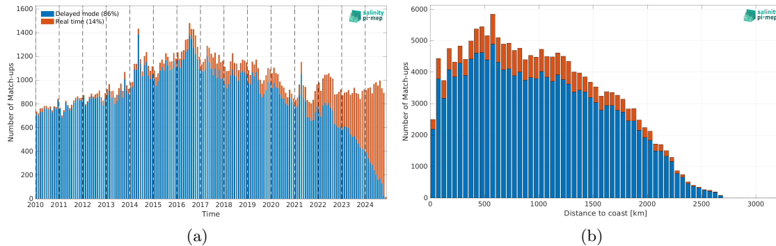
Figure 2: Number of match-ups between Argo and SMOS SSS L4 v1 - Monthly (CMEMS-CNR) SSS as a function of time (a) and as function of the distance to coast (b) over the Equatorial Ocean 10N-10S Pi-MEP region and for the full satellite product period.
