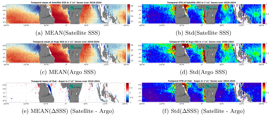
Figure 7: Temporal mean (left) and Std (right) of SSS from SMOS SSS L4 v1 - Monthly (CMEMS-CNR) (top), Argo (middle), and of \Delta SSS (Satellite - Argo). Only match-up pairs are used to generate these maps.
