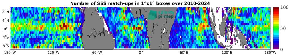
Figure 5: Number of SSS match-ups between Argo SSS and the SMOS SSS L4 v1 - Monthly (CMEMS-CNR) SSS product for the Equatorial Ocean 10N-10S Pi-MEP region over 1^\circ \times 1^\circ boxes and for the full satellite product period.
