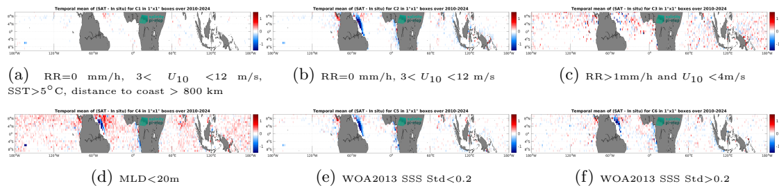
Figure 14: Temporal mean gridded over spatial boxes of size 1^\circ \times 1^\circ of \Delta SSS (SMOS SSS L4 v1 - Monthly (CMEMS-CNR) - Argo) for 6 different subdatasets corresponding to:RR=0 mm/h, 3 < U_{10} < 12 m/s, SST >5^\circ C, distance to coast > 800 km (a), RR=0 mm/h, 3 < U_{10} < 12 m/s (b), RR >1 mm/h and U_{10} < 4 m/s (c),MLD <20 m (d),WOA2013 SSS Std <0.2 (e),WOA2013 SSS Std >0.2 (f).
