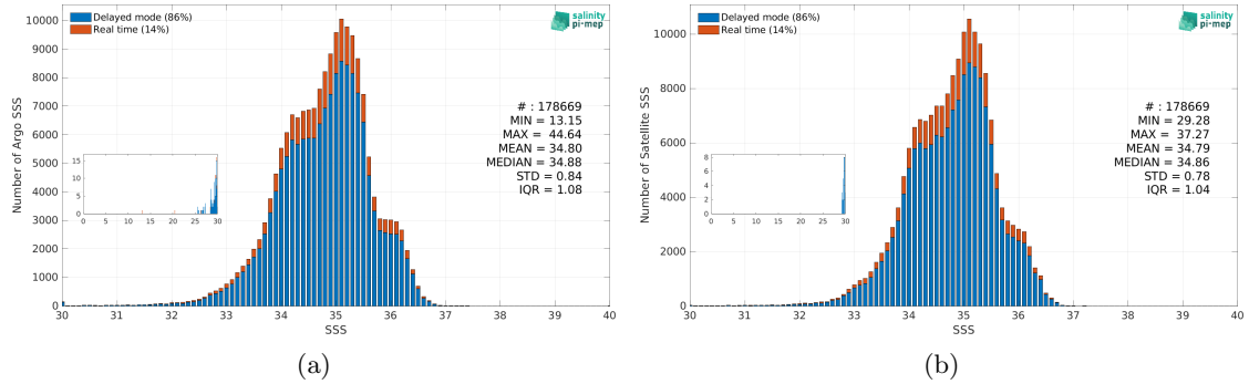
Figure 3: Histograms of SSS from Argo (a) and SMOS SSS L4 v1 - Monthly (CMEMS-CNR) (b) considering all match-up pairs per bins of 0.1 over the Equatorial Ocean 10N-10S Pi-MEP region and for the full satellite product period.
