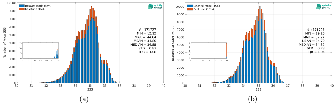
Figure 3: Histograms of SSS from Argo (a) and SMOS SSS L4 v1 - Monthly (CMEMS-CNR) (b) considering all match-up pairs per bins of 0.1 over the Equatorial Ocean 10N-10S Pi-MEP region and for the full satellite product period.
