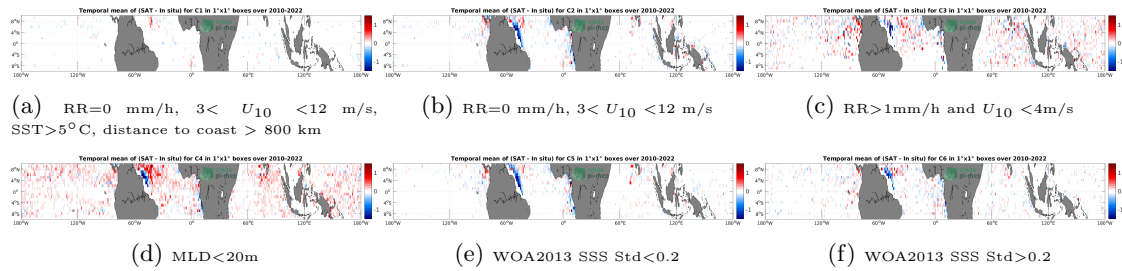
Figure 12: Temporal mean gridded over spatial boxes of size 1^\circ \times 1^\circ of \Delta SSS (SMOS SSS L4 v1 - Monthly (CMEMS-CNR) - Argo) for 6 different subdatasets corresponding to:RR=0 mm/h, 3 < U_{10} < 12 m/s, SST >5^\circ C, distance to coast > 800 km (a), RR=0 mm/h, 3 < U_{10} < 12 m/s (b), RR >1 mm/h and U_{10} < 4 m/s (c),MLD <20 m (d),WOA2013 SSS Std <0.2 (e),WOA2013 SSS Std >0.2 (f).
