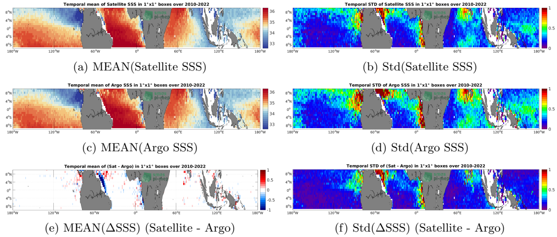
Figure 6: Temporal mean (left) and Std (right) of SSS from SMOS SSS L4 v1 - Monthly (CMEMS-CNR) (top), Argo (middle), and of \Delta SSS (Satellite - Argo). Only match-up pairs are used to generate these maps.
