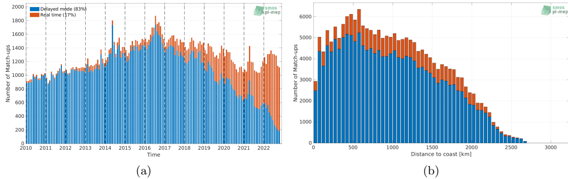
Figure 1: Number of match-ups between Argo and SMOS SSS L4 v1 - Monthly (CMEMS-CNR) SSS as a function of time (a) and as function of the distance to coast (b) over the Equatorial Ocean 10N-10S Pi-MEP region and for the full satellite product period.
