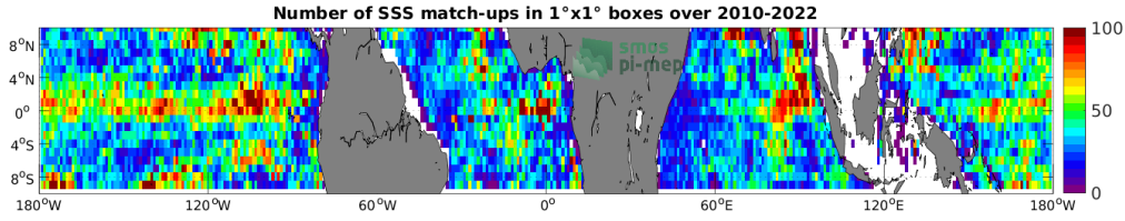
Figure 4: Number of SSS match-ups between Argo SSS and the SMOS SSS L4 v1 - Monthly (CMEMS-CNR) SSS product for the Equatorial Ocean 10N-10S Pi-MEP region over 1^\circ \times 1^\circ boxes and for the full satellite product period.
