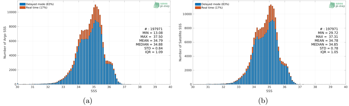
Figure 2: Histograms of SSS from Argo (a) and SMOS SSS L4 v1 - Monthly (CMEMS-CNR) (b) considering all match-up pairs per bins of 0.1 over the Equatorial Ocean 10N-10S Pi-MEP region and for the full satellite product period.
