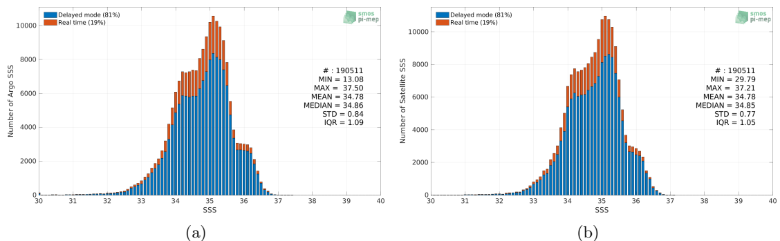
Figure 2: Histograms of SSS from Argo (a) and SMOS SSS L4 v1 - Monthly (CMEMS-CNR) (b) considering all match-up pairs per bins of 0.1 over the Equatorial Ocean 10N-10S Pi-MEP region and for the full satellite product period.
