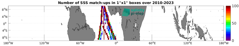
Figure 5: Number of SSS match-ups between TSG (Polarstern) SSS and the SMOS SSS L4 v1 - Daily (CMEMS-CNR) SSS product for the Equatorial Ocean 10N-10S Pi-MEP region over 1^\circ \times 1^\circ boxes and for the full satellite product period.
