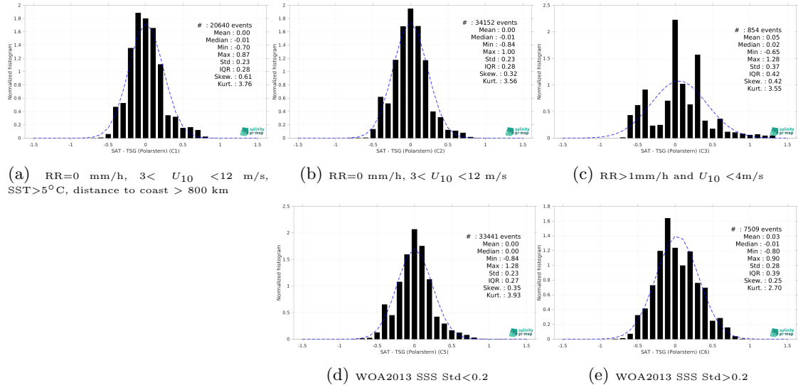
Figure 15: Normalized histogram of \Delta SSS (SMOS SSS L4 v1 - Daily (CMEMS-CNR) - TSG (Polarstern)) for 5 different subdatasets corresponding to: RR=0 mm/h, 3 < U_{10} < 12 m/s, SST>5°C, distance to coast > 800 km (a), RR=0 mm/h, 3 < U_{10} < 12 m/s (b), RR>1mm/h and U_{10} < 4 m/s (c), WOA2013 SSS Std<0.2 (d), WOA2013 SSS Std>0.2 (e).
