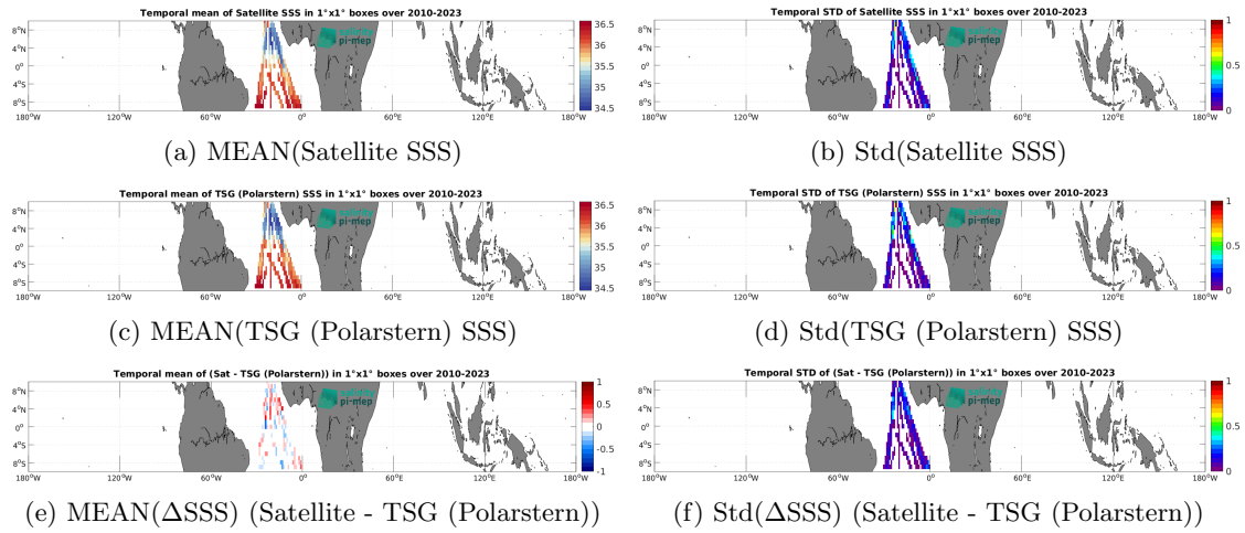
Figure 7: Temporal mean (left) and Std (right) of SSS from SMOS SSS L4 v1 - Daily (CMEMS-CNR) (top), TSG (Polarstern) (middle), and of \Delta SSS (Satellite - TSG (Polarstern)). Only match-up pairs are used to generate these maps.
