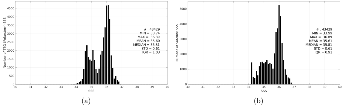
Figure 3: Histograms of SSS from TSG (Polarstern) (a) and SMOS SSS L4 v1 - Daily (CMEMS-CNR) (b) considering all match-up pairs per bins of 0.1 over the Equatorial Ocean 10N-10S Pi-MEP region and for the full satellite product period.
