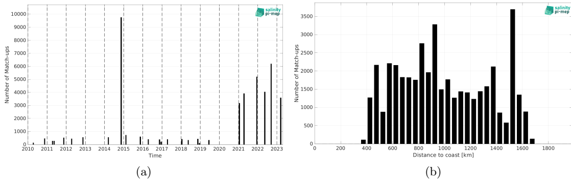
Figure 2: Number of match-ups between TSG (Polarstern) and SMOS SSS L4 v1 - Daily (CMEMS-CNR) SSS as a function of time (a) and as function of the distance to coast (b) over the Equatorial Ocean 10N-10S Pi-MEP region and for the full satellite product period.
