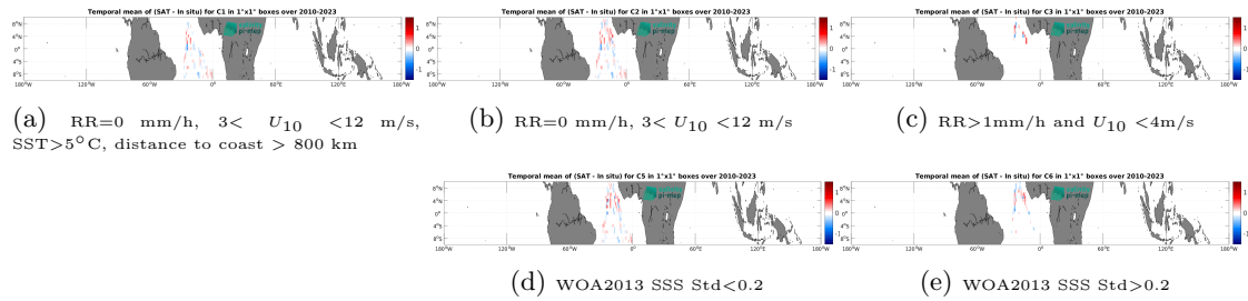
Figure 14: Temporal mean gridded over spatial boxes of size 1^\circ \times 1^\circ of \Delta SSS (SMOS SSS L4 v1 - Daily (CMEMS-CNR) - TSG (Polarstern)) for 5 different subdatasets corresponding to: RR=0 mm/h, 3 < U_{10} < 12 m/s, SST>5°C, distance to coast > 800 km (a), RR=0 mm/h, 3 < U_{10} < 12 m/s (b), RR>1mm/h and U_{10} < 4 m/s (c), WOA2013 SSS Std<0.2 (d), WOA2013 SSS Std>0.2 (e).
