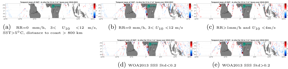
Figure 14: Temporal mean gridded over spatial boxes of size 1^\circ \times 1^\circ of \Delta SSS (SMOS SSS L4 v1 - Daily (CMEMS-CNR) - TSG (LEGOS-DM)) for 5 different subdatasets corresponding to: RR=0 mm/h, 3 < U_{10} < 12 m/s, SST>5°C, distance to coast > 800 km (a), RR=0 mm/h, 3 < U_{10} < 12 m/s (b), RR>1mm/h and U_{10} < 4 m/s (c), WOA2013 SSS Std<0.2 (d), WOA2013 SSS Std>0.2 (e).
