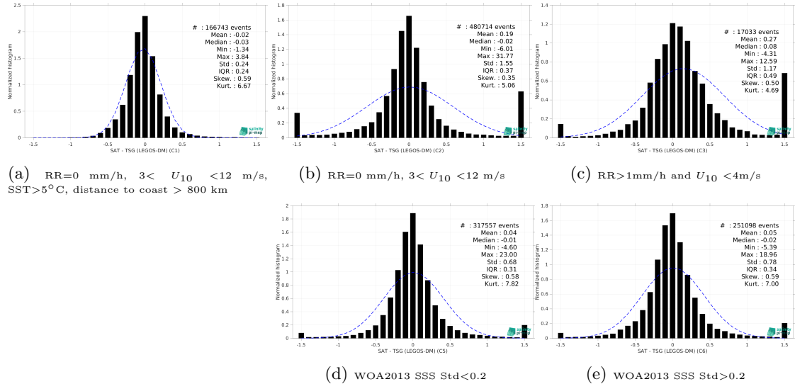
Figure 15: Normalized histogram of \Delta SSS (SMOS SSS L4 v1 - Daily (CMEMS-CNR) - TSG (LEGOS-DM)) for 5 different subdatasets corresponding to: RR=0 mm/h, 3 < U_{10} < 12 m/s, SST>5°C, distance to coast > 800 km (a), RR=0 mm/h, 3 < U_{10} < 12 m/s (b), RR>1mm/h and U_{10} < 4 m/s (c), WOA2013 SSS Std<0.2 (d), WOA2013 SSS Std>0.2 (e).
